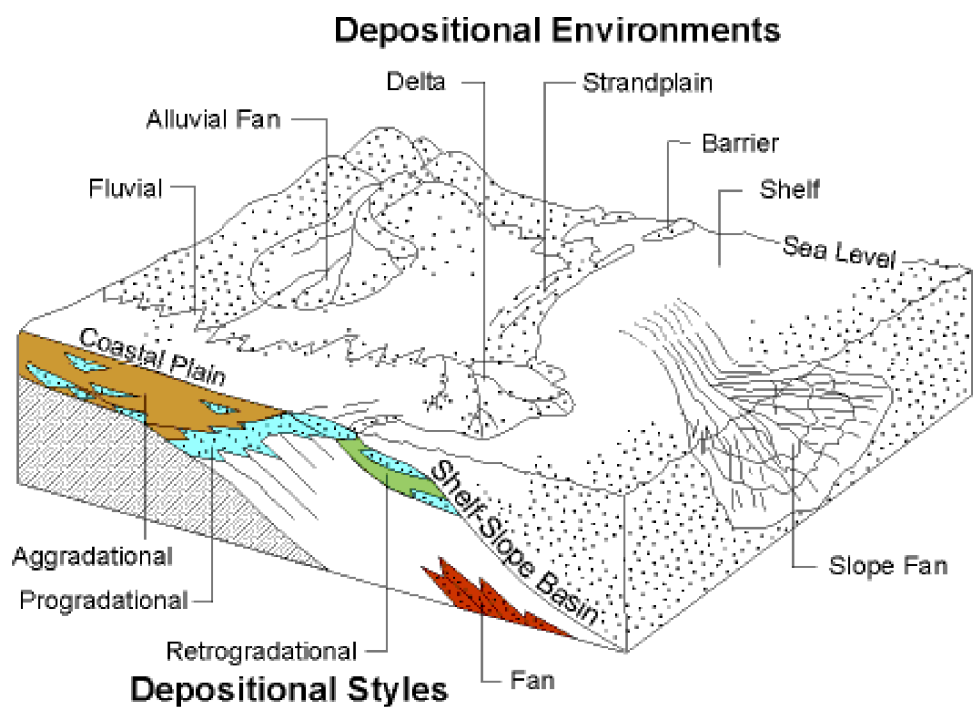
Figure 4. Block Diagram of Siliciclastic Depositional Environments that Host Hydrocarbons (GOM).
