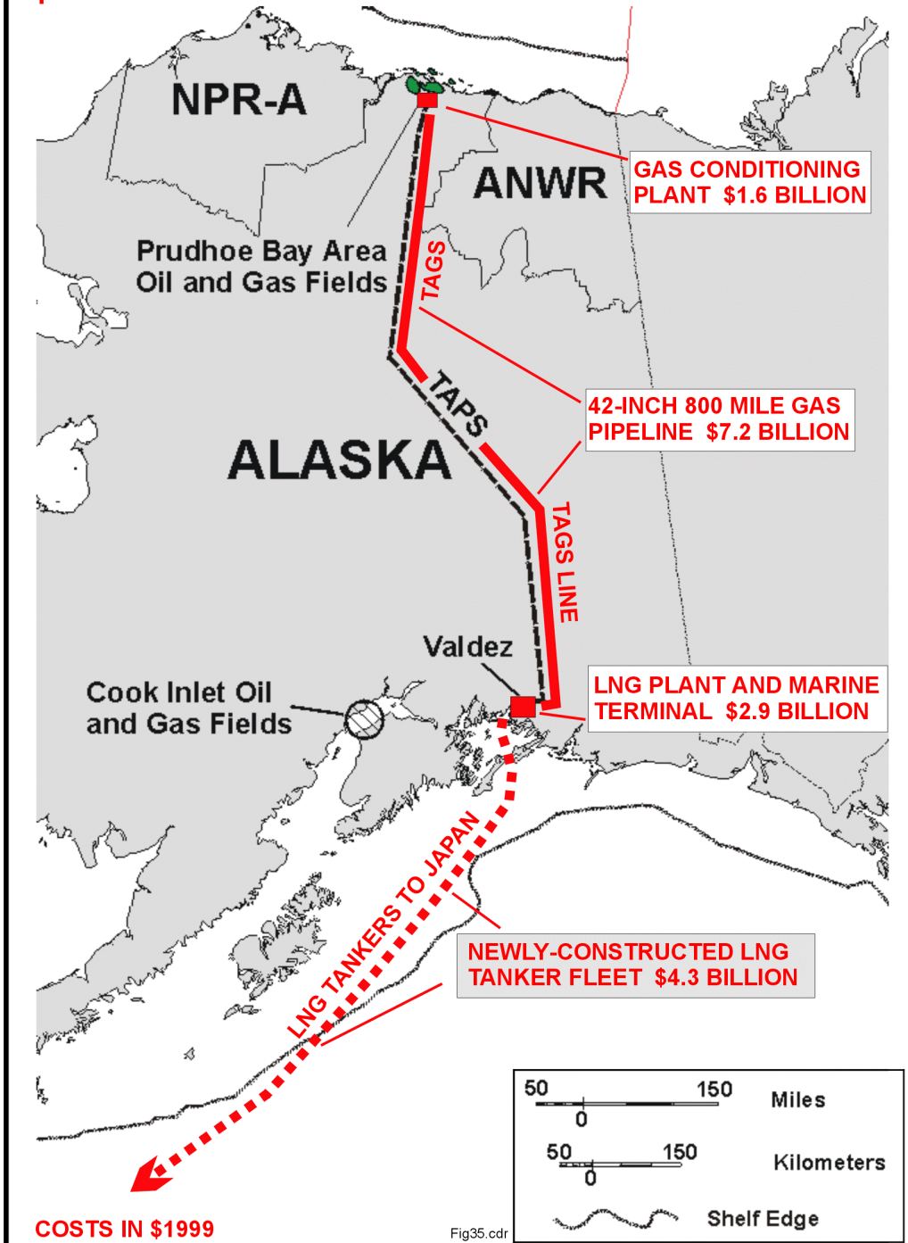
Figure 35: Elements of proposed TAGS-LNG gas transportation system requiring capital outlays for initiation of project. Cost estimates for 14 million metric ton (0.7 tcf) per year project from Thomas and others (1996, p. B-20 to B-21), with reported $1995 costs adjusted to $1999.
