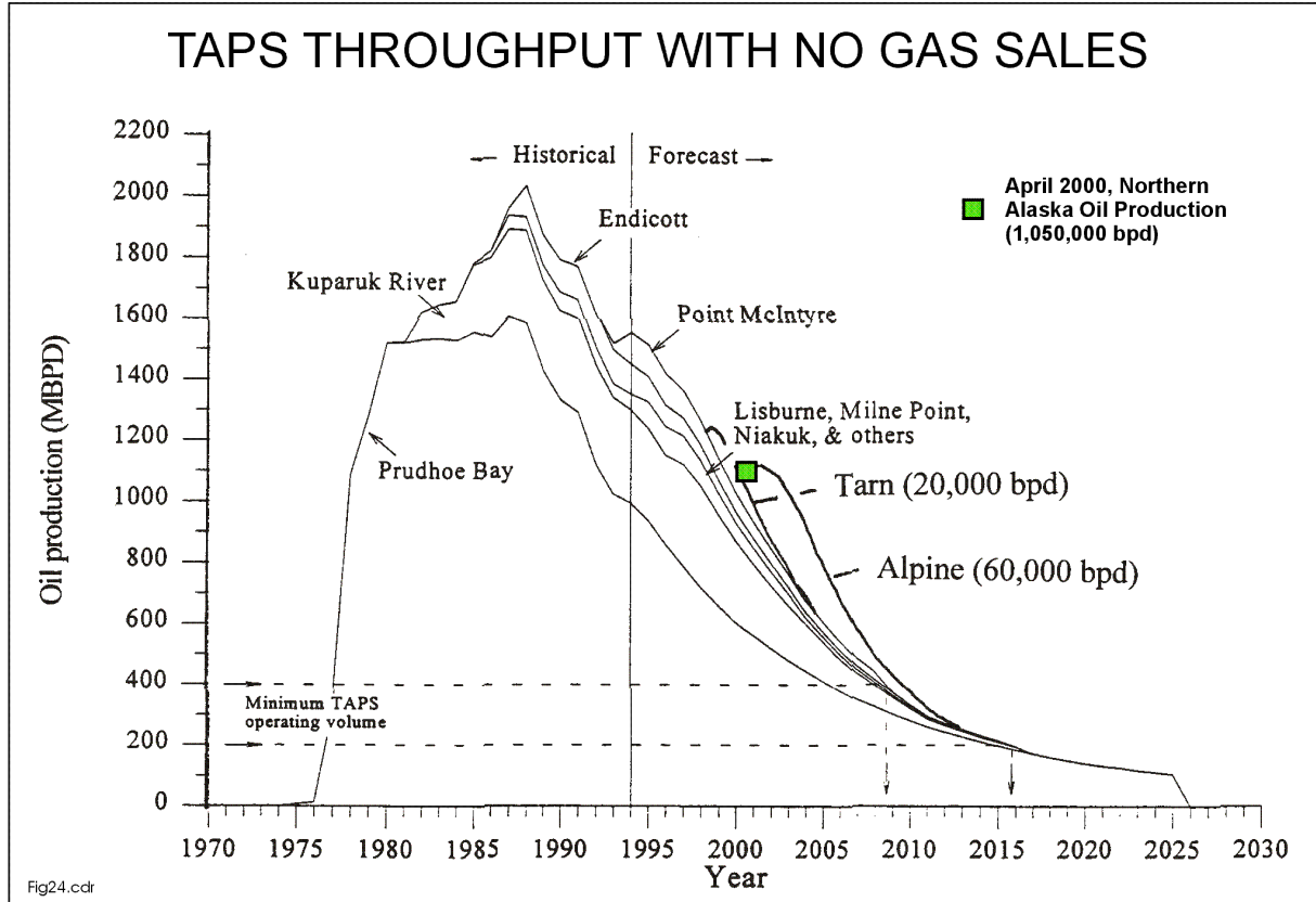
Figure 24: Production decline projections for northern Alaska producing fields in Prudhoe Bay area. Contributions from new fields at Tarn and Alpine have been added as sketches based on estimates for maximum production rates. These new fields, although significant, will not materially prolong the economic life of TAPS, projected to end when throughput falls to some level between 400,000 bpd (year 2009) and 200,000 bpd (year 2016). Diagram modified after Thomas and others (1996, fig. 2).
