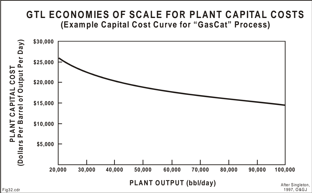
Figure 32: Example from "GasCat" process showing how larger GTL plants benefit from economy of scale and can produce liquids from gas more cheaply. For example, capital costs for this type of GTL plant, when designed for an output capacity of 100,000 barrels of liquid product per day, are only $15,000/barrel/day, nearly half the costs of plants with capacities smaller than 20,000 barrels per day. Diagram redrawn from Singleton (1997, fig. 3).
