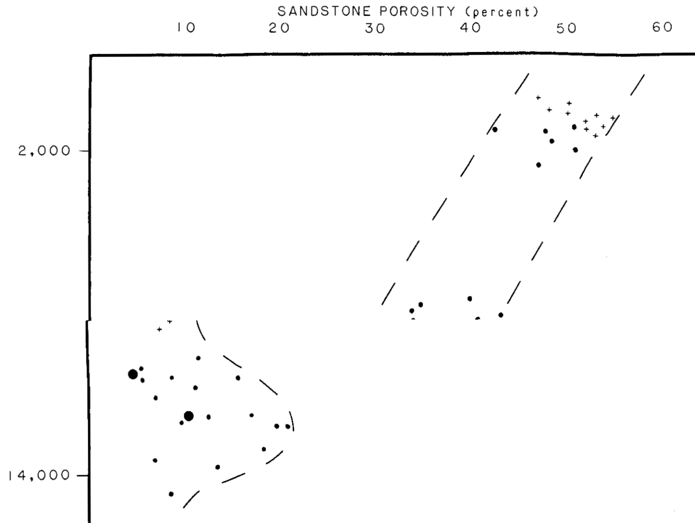
FIGURE 24. Distribution of sandstone porosity with depth, Norton Basin COST No.1 and No. 2 wells. Porosity calculated from Compensated Formation Density log data and conventional core measurements.
