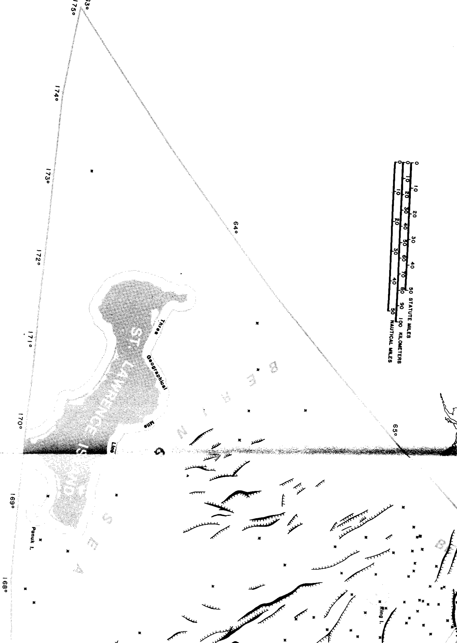
FIGURE 42. Locations of epicenters of earthquakes recorded by the local seis in relation to structural and geographic features.
