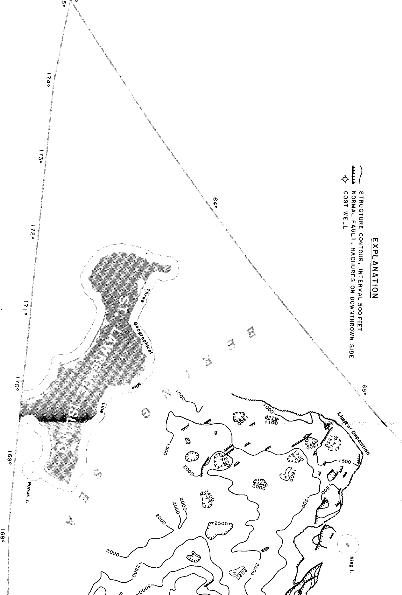
FIGURE 18. Structure contours (in depth) on horizon D in Norton Basin. Interpretation and time-depth relationship derived from W
