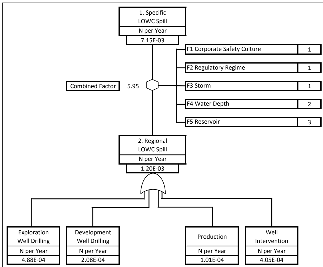
Figure 8.5: Quantified Specific Development LOWC Characteristic Evaluation Fault Tree
