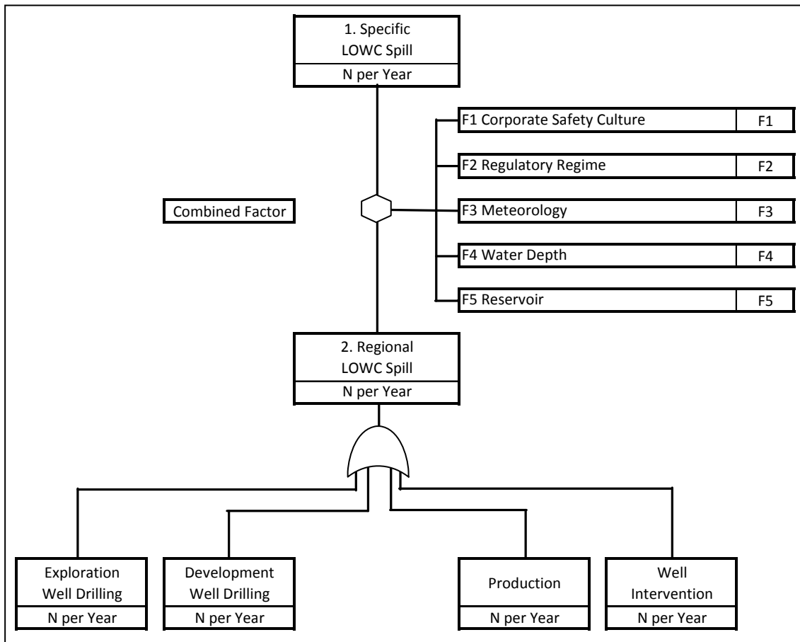
Figure 8.4: Specific Development LOWC Characteristic Evaluation Conceptual Fault Tree
