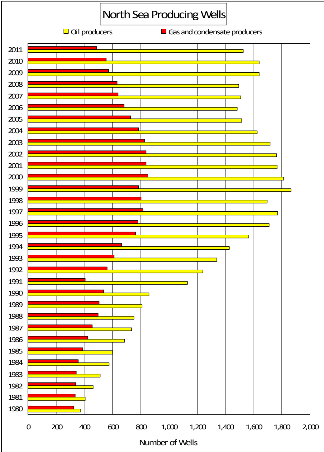
Figure 4.2: North Sea Annual Producing Well Exposure
