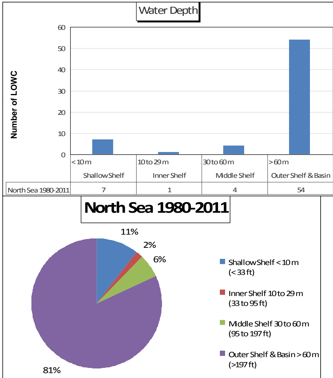
Figure 4.7: North Sea Shelf Water Depth Range LOWC Incident Distribution Graphs
