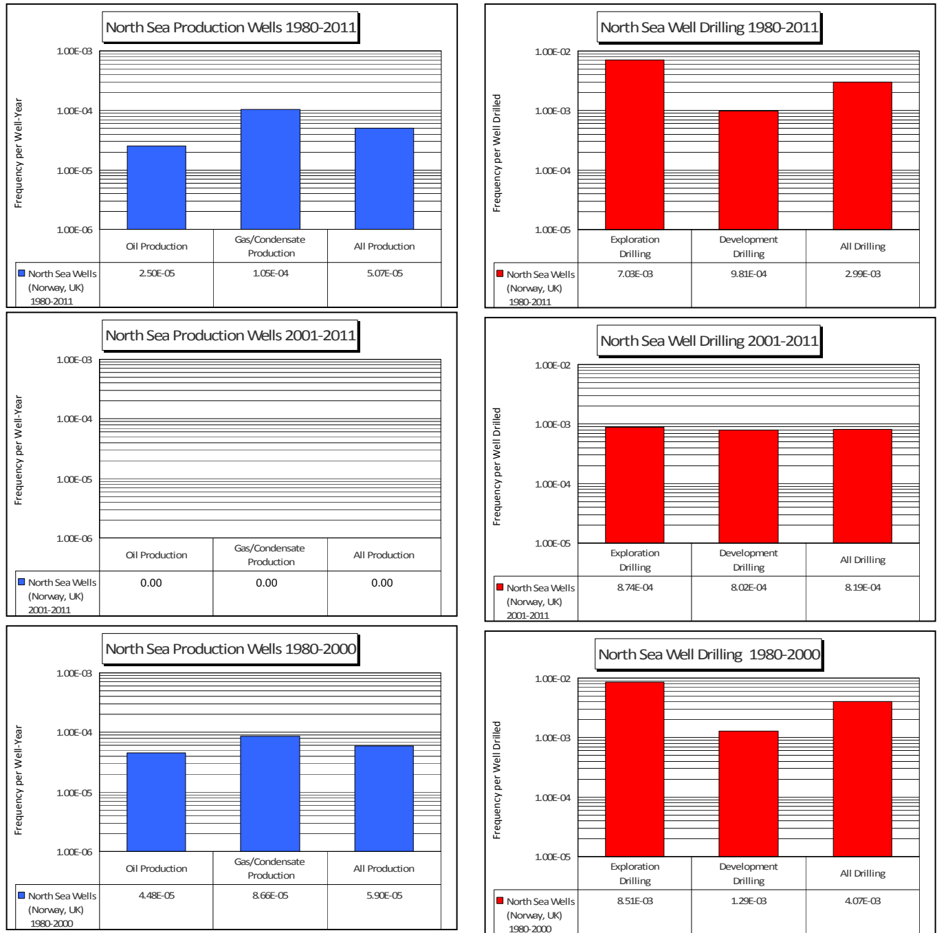
Figure 7.3: North Sea Temporal LOWC Frequency Comparisons
