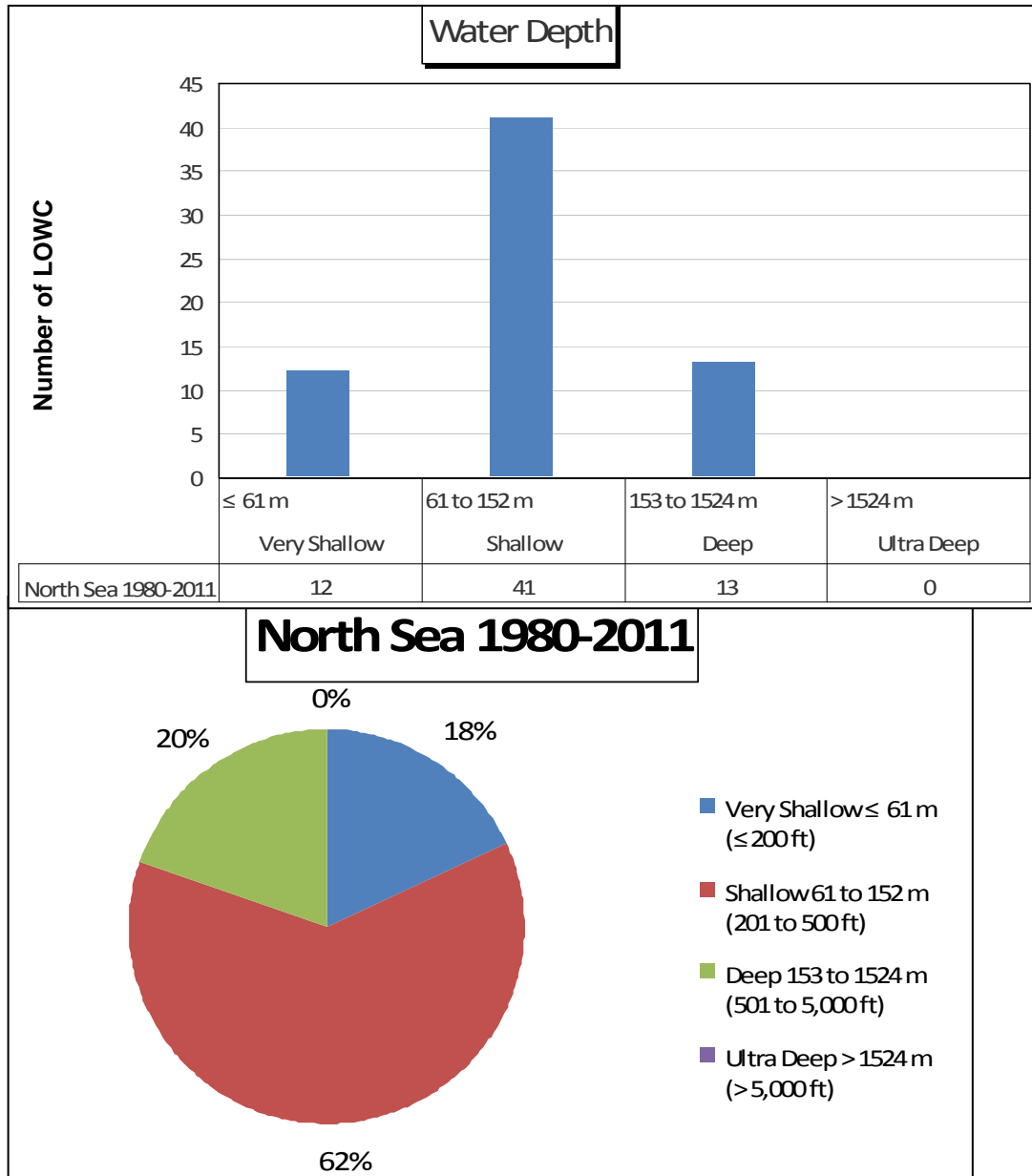
Figure 4.8: North Sea Offshore Water Depth Range LOWC Incident Distribution Graphs
