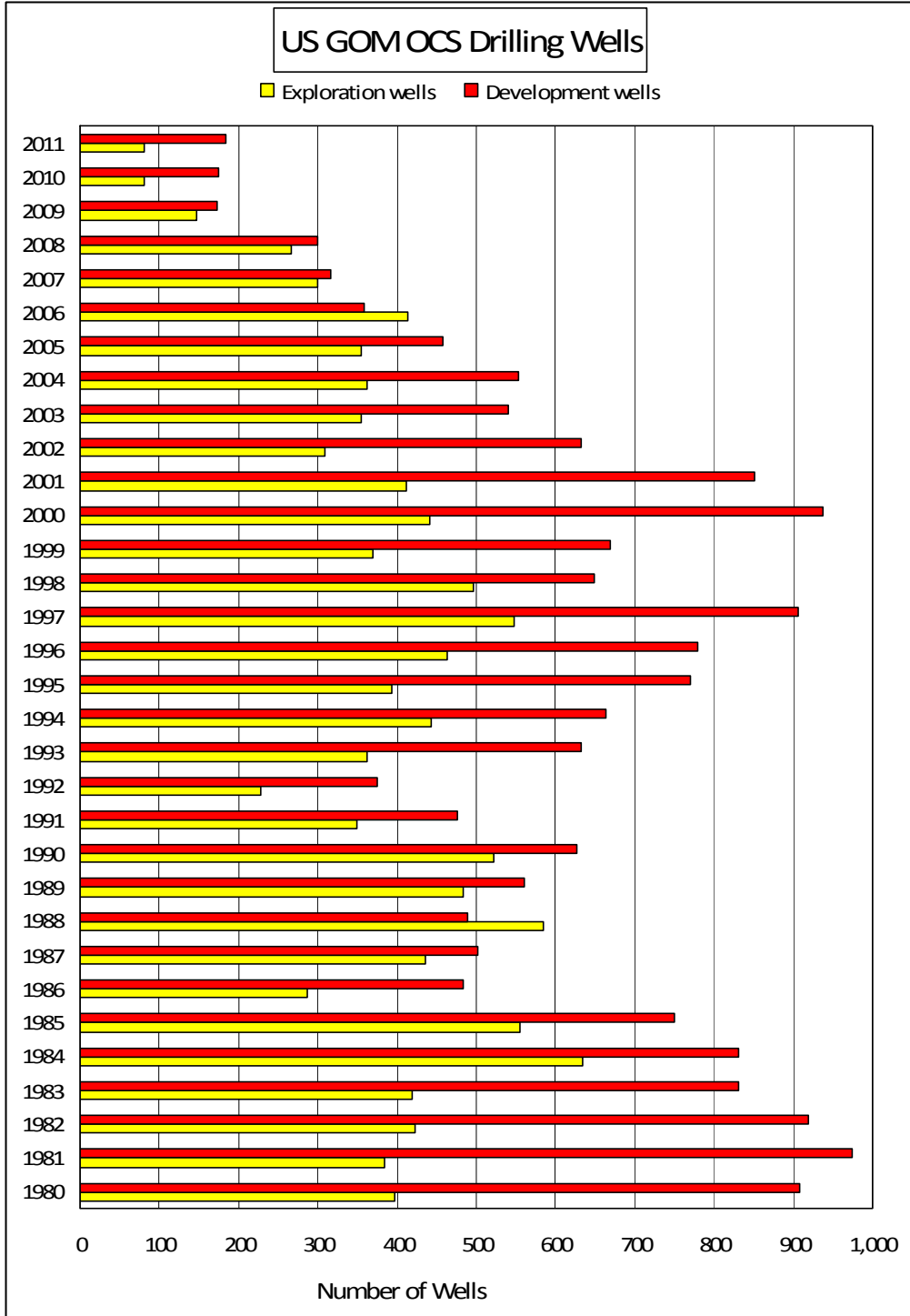
Figure 3.1: U.S. GOM Annual Well Drilling Exposure
