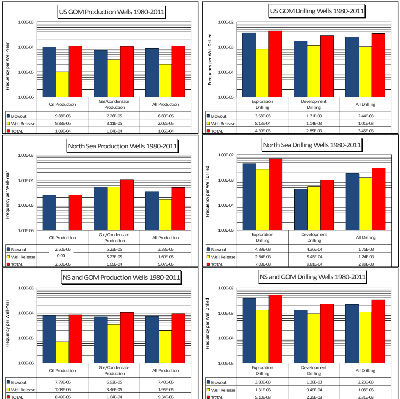
Figure 7.1: Frequency Graphs: GOM and North Sea (1980-2011)
