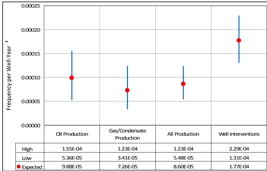
Figure 3.3: Blowout Frequency – U.S. GOM OCS Production Variability (1980-2011)
