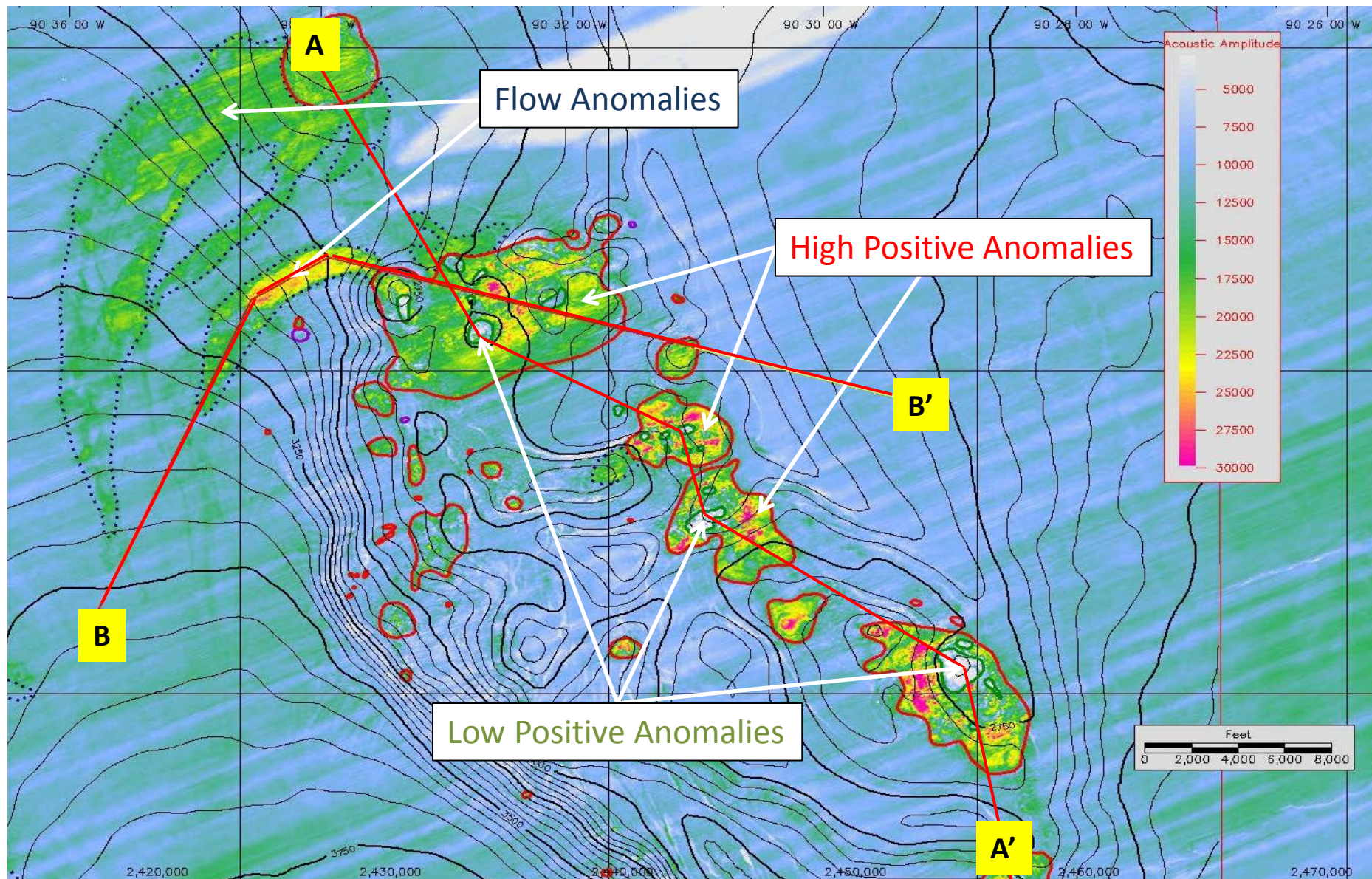
Fig. 2 – Bathymetry/Amplitude Map Showing High and Low Positive Anomalies and Flow Amplitude Anomalies
