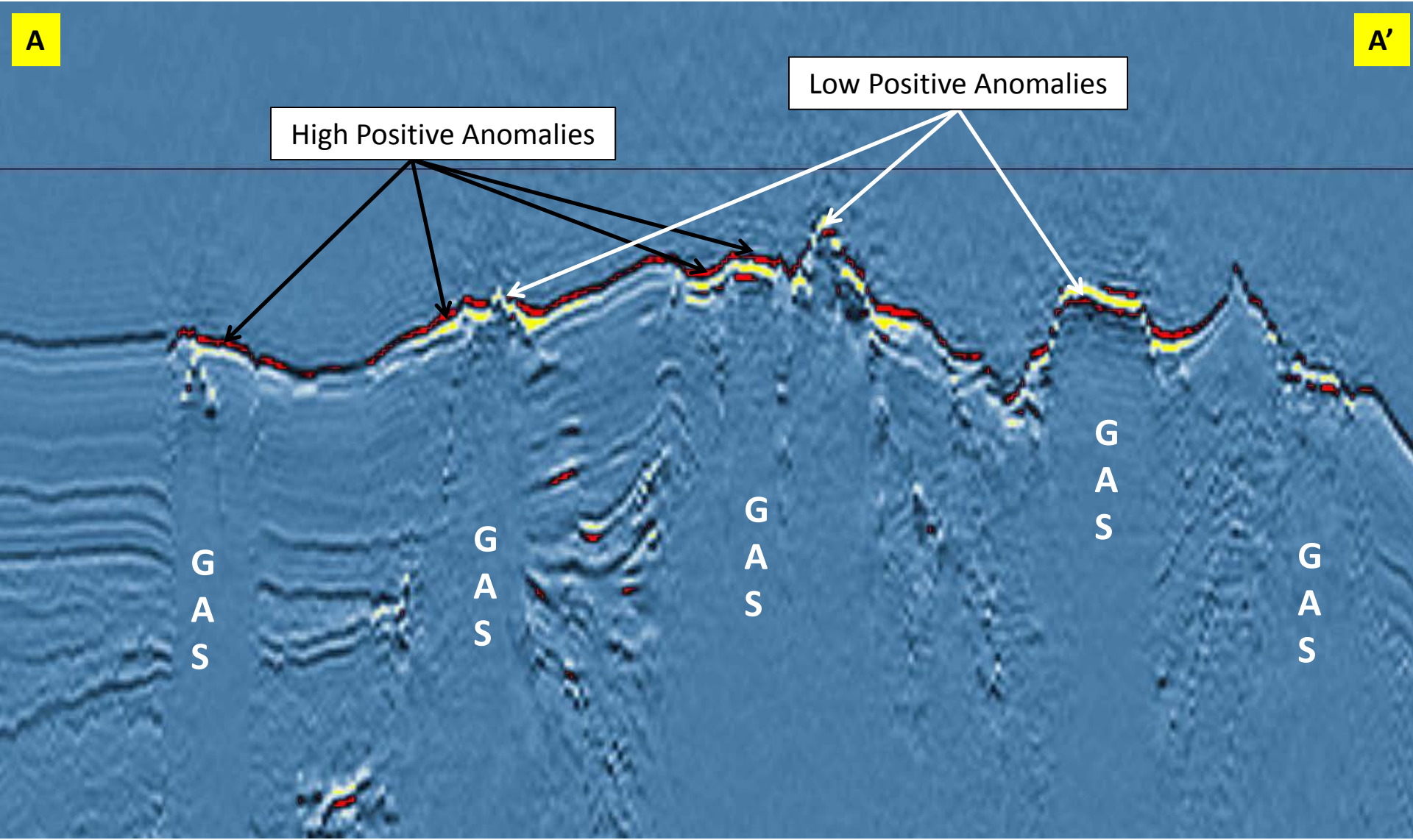
Fig. 3 – Seismic Traverse A-A' Showing High and Low Positive Amplitude Anomalies
