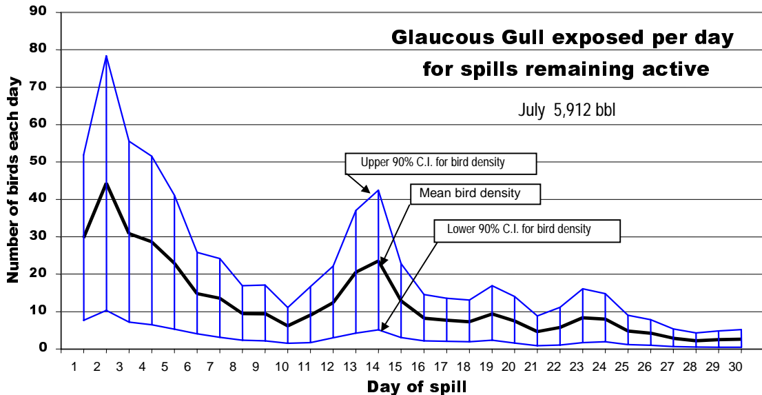
Figure 10. Number of glaucous gull exposed in 500 trajectories of 5912-barrel spills in July.
