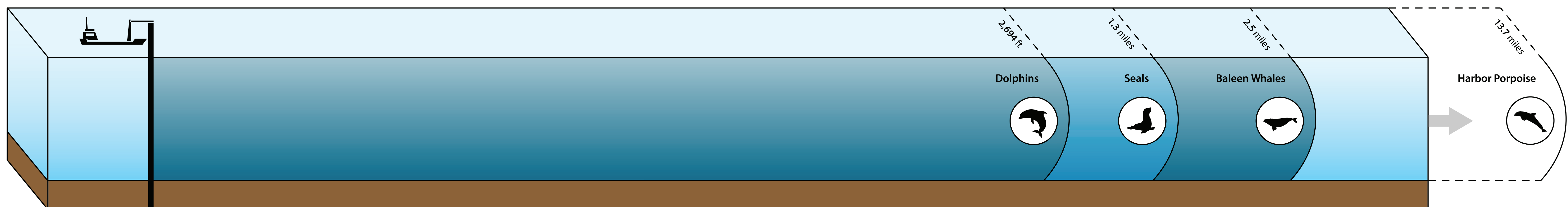
Distances to a 50% adverse behavioral disturbance for marine mammals at 160 dB RMS. Distances are adjusted for hearing sensitivity for animal groups shown.
