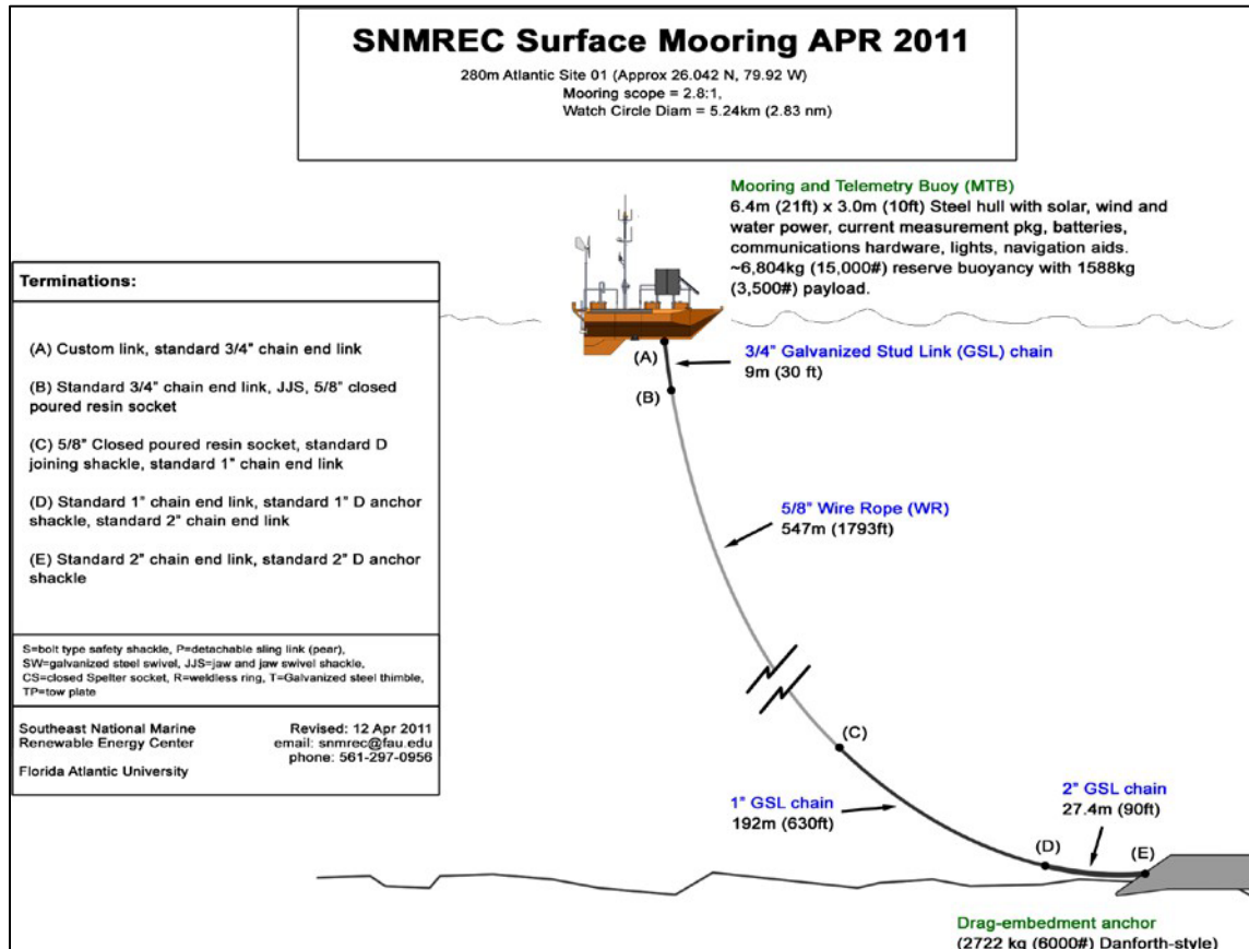
Figure 2.2. MTB mooring system.
