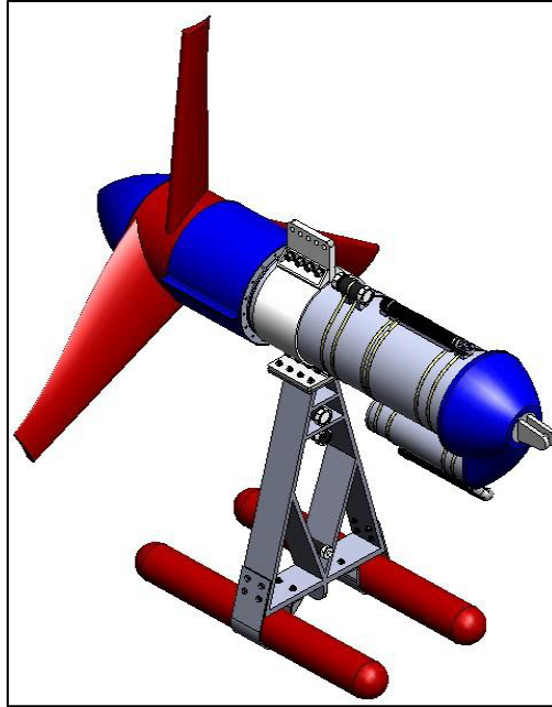
Figure 2.3. Testing device. (Source: FAU, 2011)
