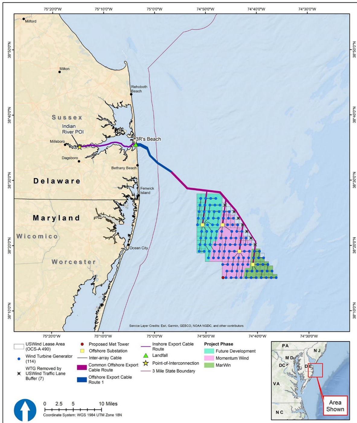
Figure 2-1. Maryland Offshore Wind Project
