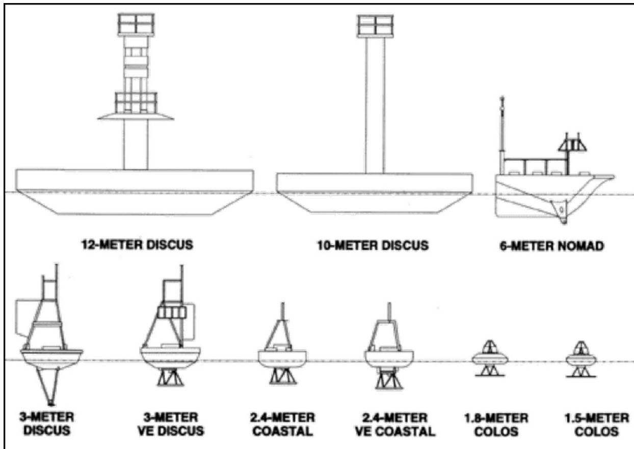
Figure 3-7 Buoy Schematic
