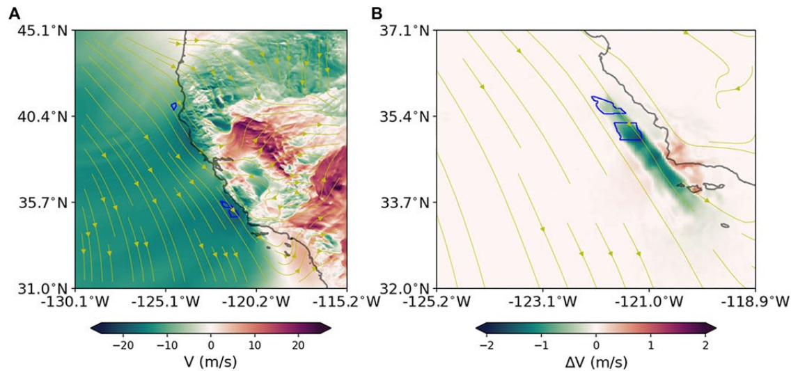
Figure 1. (A) Hub-height wind field on 15 Apr 2000; and (B) change in wind wake (green) due to one scenario of future wind farms. Note the O(1-2 \text{ m/s}) wind speed reduction behind the Morro Bay wind energy area of interest, which would potentially reduce upwelling. From Raghukumar et al. (2022).
