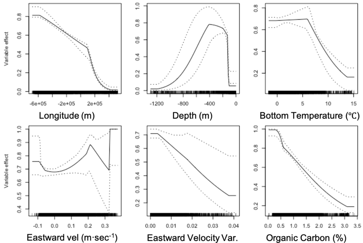
Figure 3.26. Response Curves for the Most Influential Habitat Covariates in the MaxEnt Model Predicting Probability of Suitable Habitat for Adolescent Male Snow Crab
