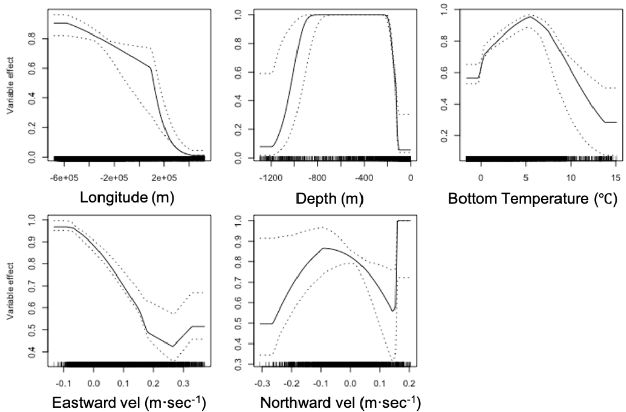
Figure 3.28. Response Curves for the Most Influential Habitat Covariates in the MaxEnt Model Predicting Probability of Suitable Habitat for Mature Female Snow Crab
