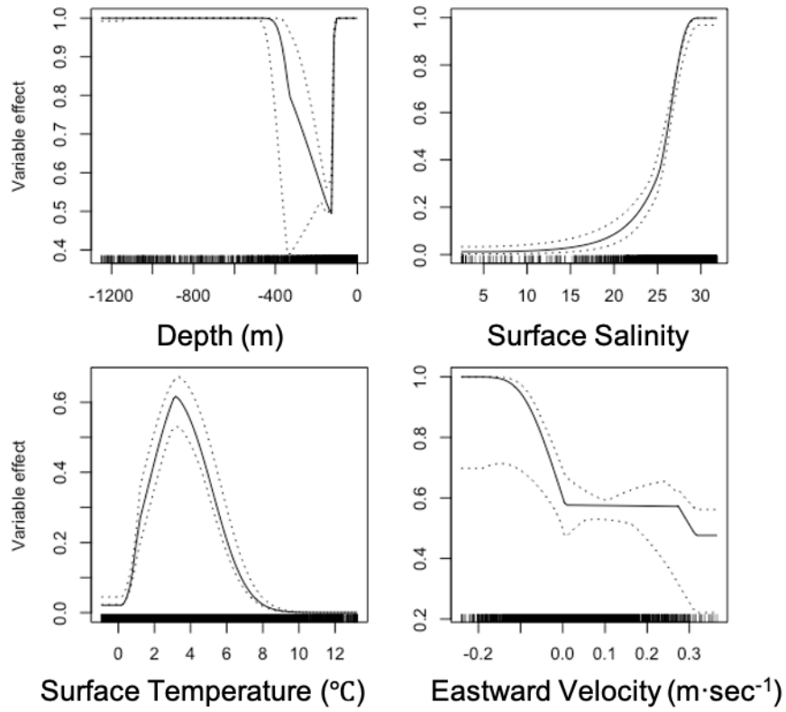
Figure 3.3. Response Curves for the Most Influential Habitat Covariates in the MaxEnt Model Predicting Probability of Suitable Habitat for Larval Arctic Cod
