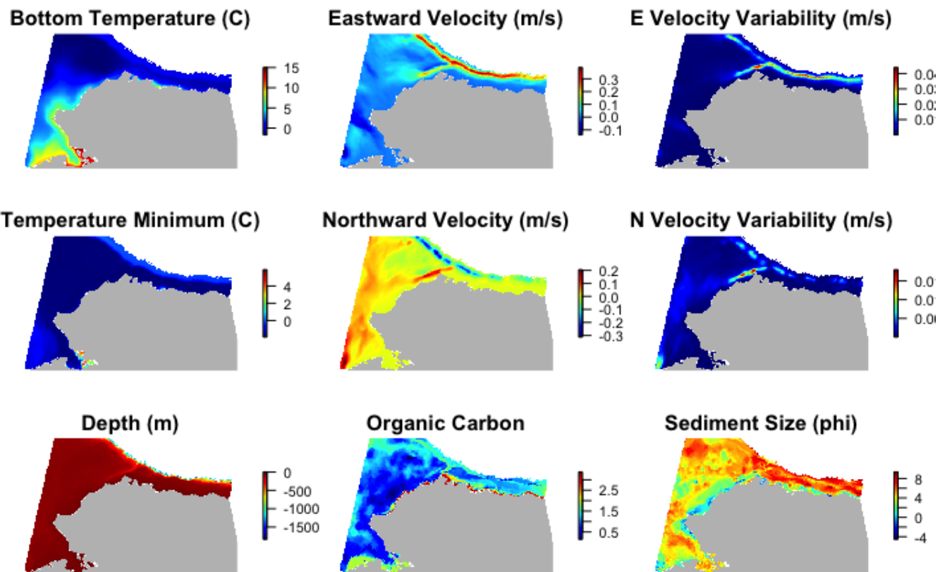
Figure 2.3. Near Bottom Habitat Covariate Rasters (Explanatory Variables)
