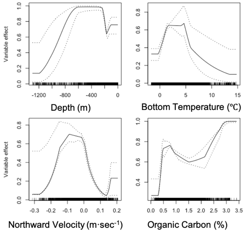
Figure 3.7. Response Curves for the Most Influential Habitat Covariates in the MaxEnt Model Predicting Probability of Suitable Habitat for Juvenile Arctic Cod
