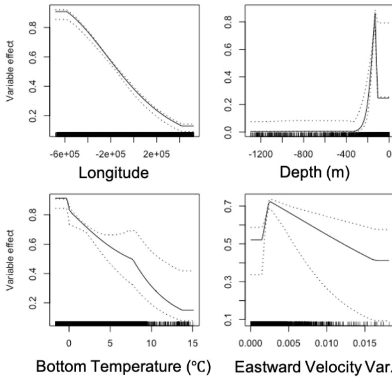
Figure 3.22. Response Curves for the Most Influential Habitat Covariates in the MaxEnt Model Predicting Probability of Suitable Habitat for Immature Snow Crab
