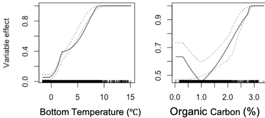
Figure 3.16. Response Curves for the Most Influential Habitat Covariates in the MaxEnt Model Predicting Probability of Suitable Habitat for Juvenile Saffron Cod
