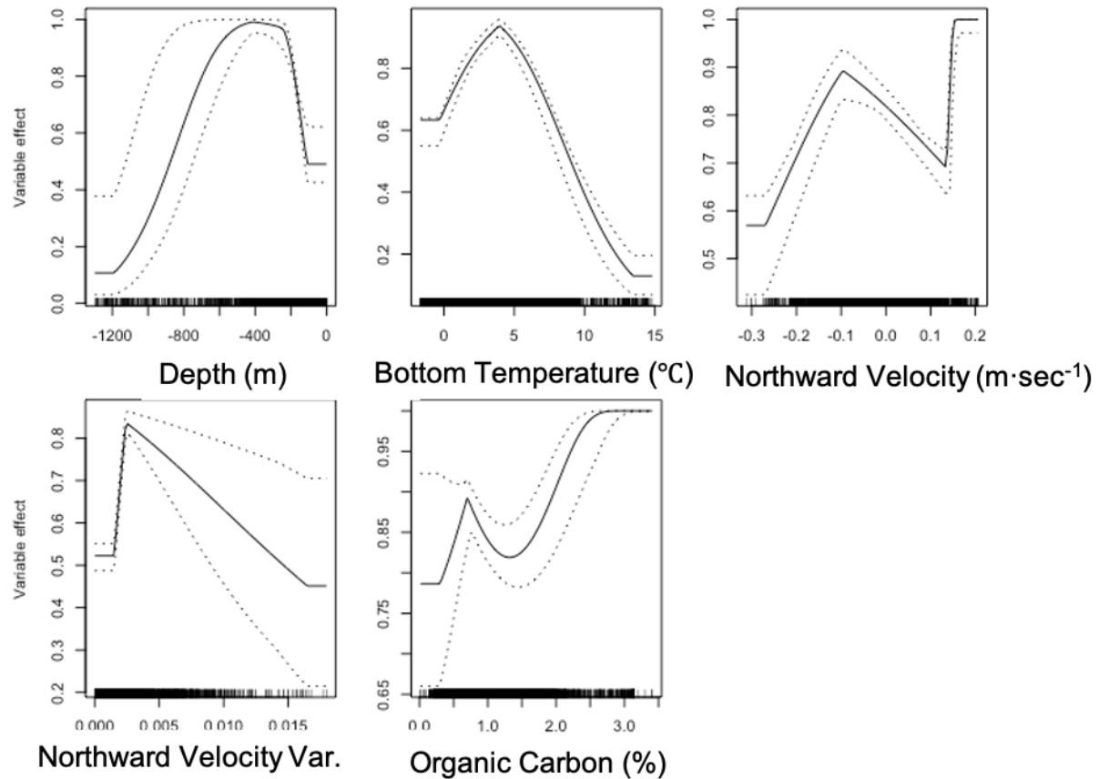
Figure 3.9. Response Curves for the Most Influential Habitat Covariates in the MaxEnt Model Predicting Probability of Suitable Habitat for Mature Arctic Cod
