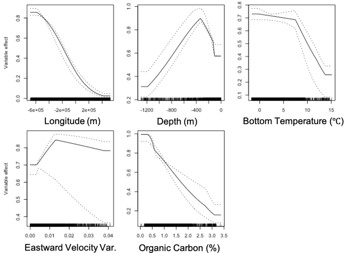
Figure 3.24. Response Curves for the Most Influential Habitat Covariates in the MaxEnt Model Predicting Probability of Suitable Habitat for Adolescent Female Snow Crab
