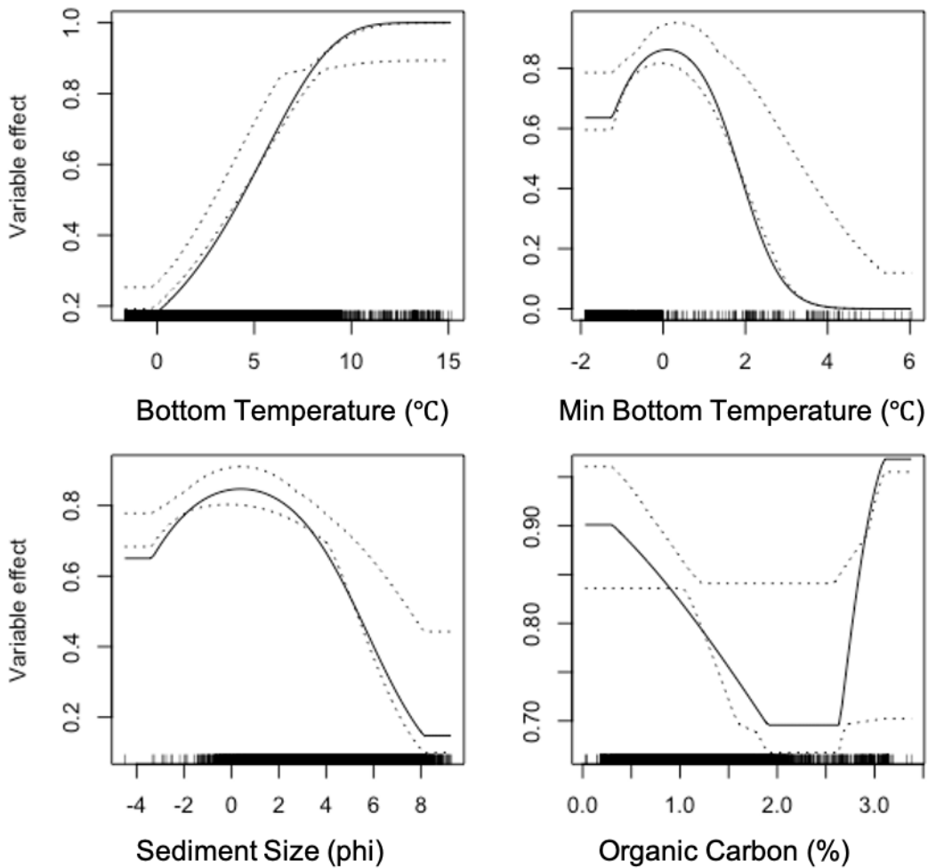
Figure 3.18. Response Curves for the Most Influential Habitat Covariates in the MaxEnt Model Predicting Probability of Suitable Habitat for Mature Saffron Cod
