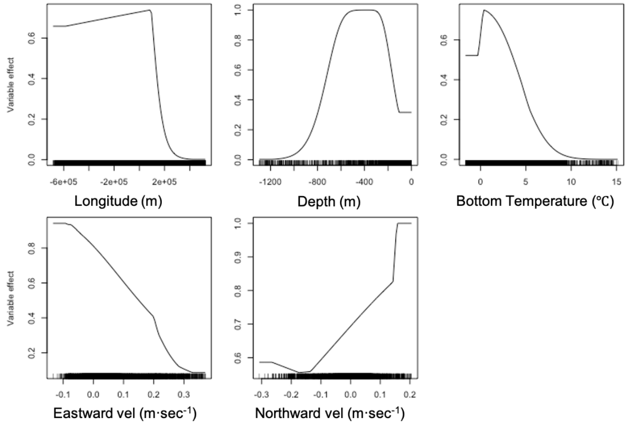
Figure 3.30. Response Curves for the Most Influential Habitat Covariates in the MaxEnt Model Predicting Probability of Suitable Habitat for Mature Male Snow Crab
