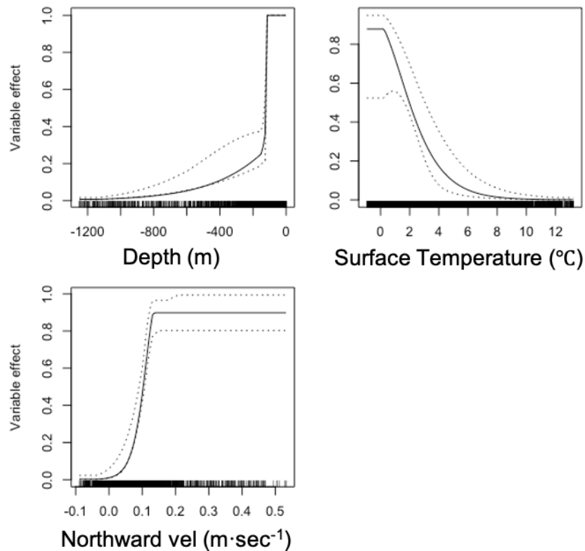
Figure 3.12. Response Curves for the Most Influential Habitat Covariates in the MaxEnt Model Predicting Probability of Suitable Habitat for Larval Saffron Cod
