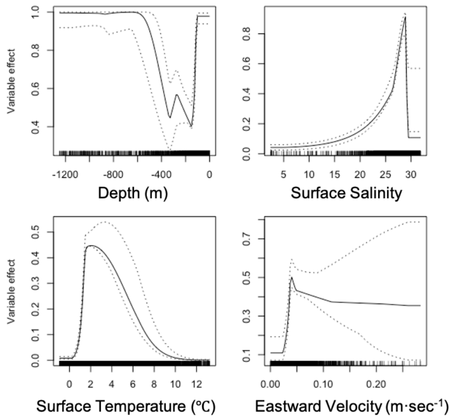
Figure 3.5. Response Curves for the Most Influential Habitat Covariates in the MaxEnt Model Predicting Probability of Suitable Habitat for Age 0 Arctic Cod
