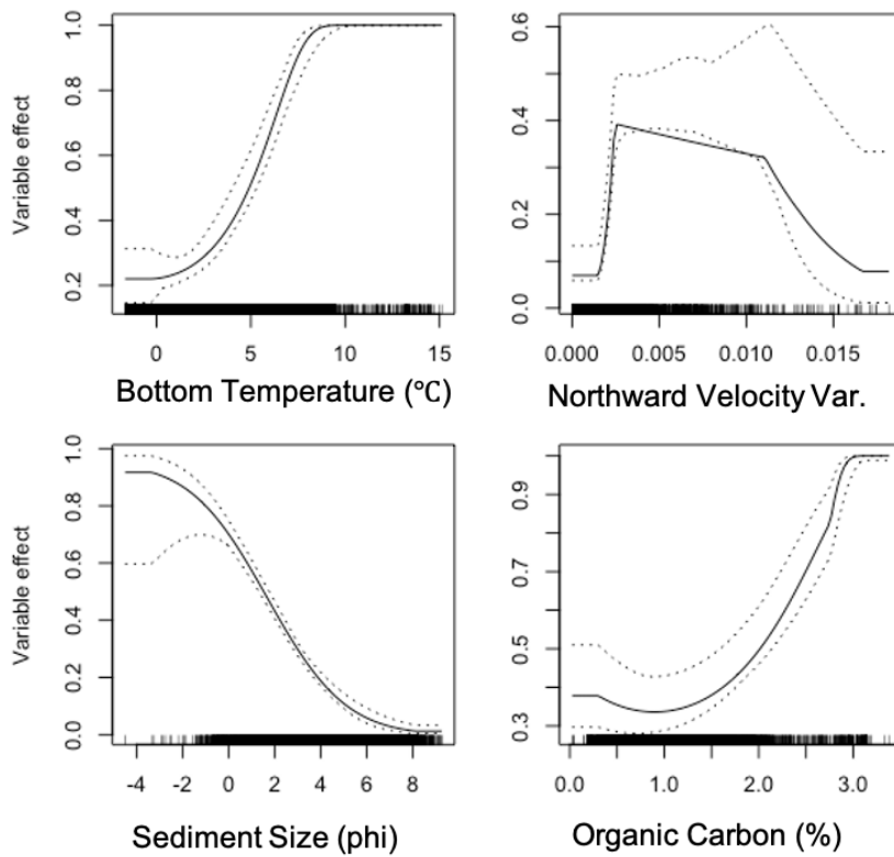
Figure 3.14. Response Curves for the Most Influential Habitat Covariates in the MaxEnt Model Predicting Probability of Suitable Habitat for Age 0 Saffron Cod
