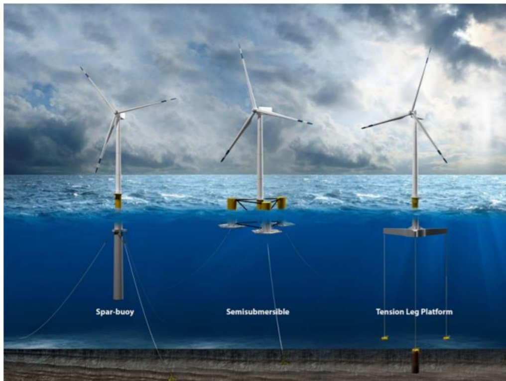
Figure 1. Floating offshore wind substructure topologies including spar-buoy, semisubmersible, and tension leg platform. Illustration by Josh Bauer, NREL.
