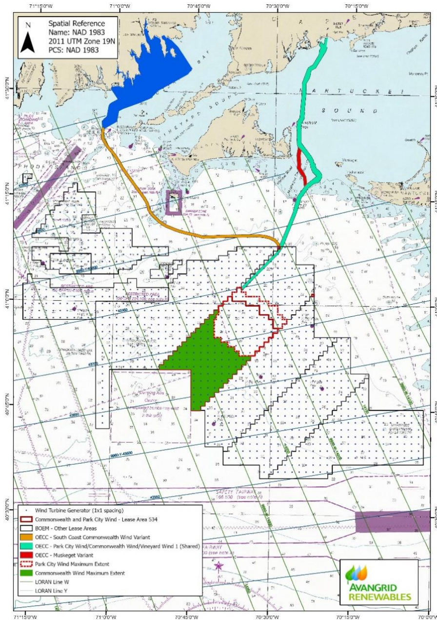
Figure 2. OECC for Park City Wind and Commonwealth Wind
