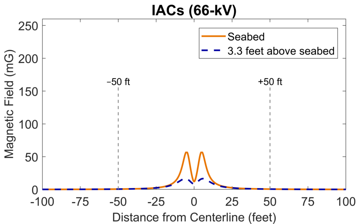
Figure C-1. Calculated magnetic-field levels in seawater above the IACs for a 3.3-foot burial depth and average loading.
