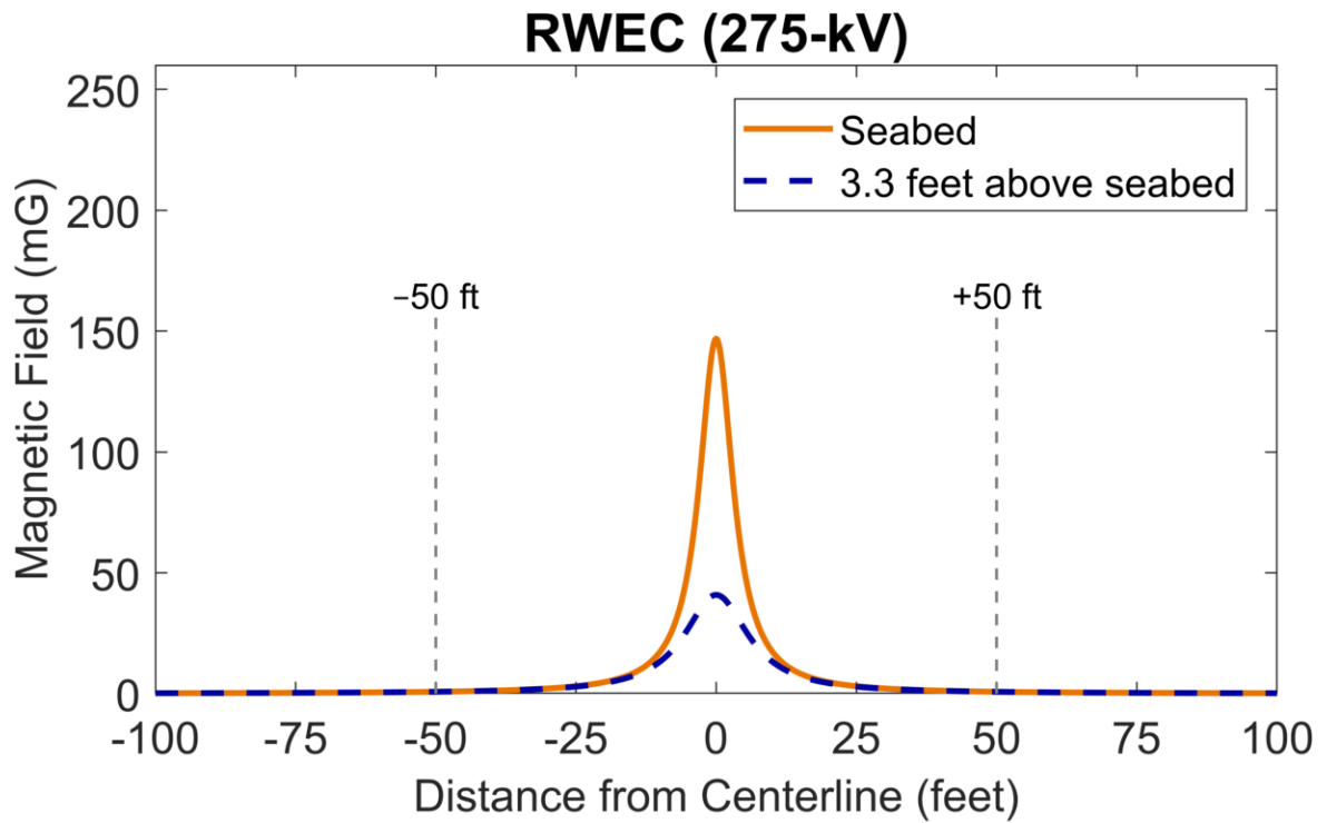
Figure C-2. Calculated magnetic-field levels in seawater above the RWEK for a 3.3-foot burial depth and average loading.
