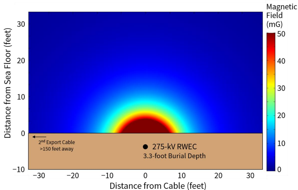
Figure 3. Calculated magnetic-field levels in seawater above the 275-kV RWE for a 3.3-foot (1 m) burial depth and average loading.
