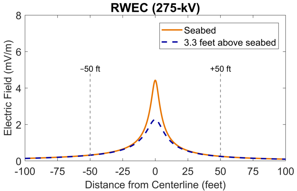
Figure C-5. Calculated induced electric-field levels in seawater above the RWEC for a 3.3-foot burial depth and average loading.
