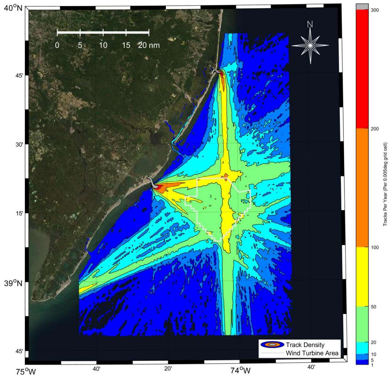
Figure 6.18: AIS Vessel Traffic Density for Fishing Vessels (> 4 Knots) for those Vessels that have Entered the WTA
