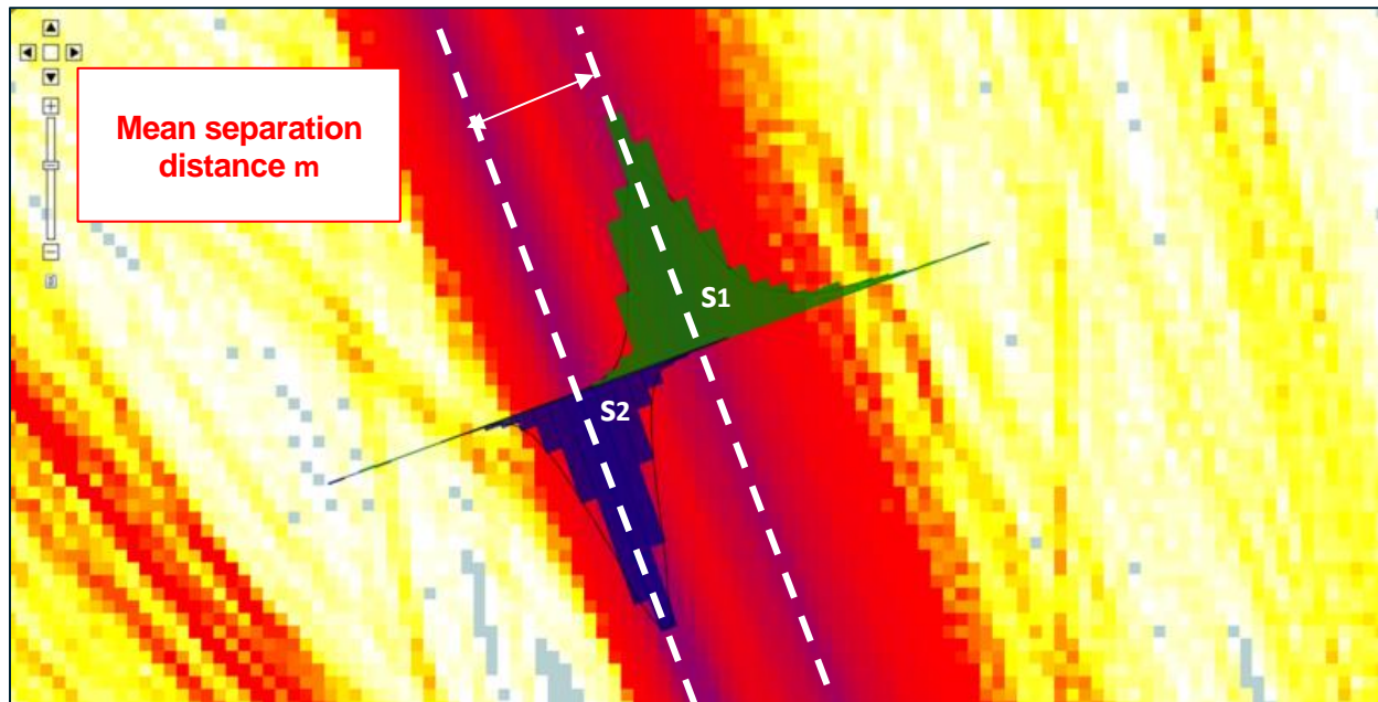
Figure E.2: Spatial Distribution of Traffic Concentration and Vessel Traffic Distribution
