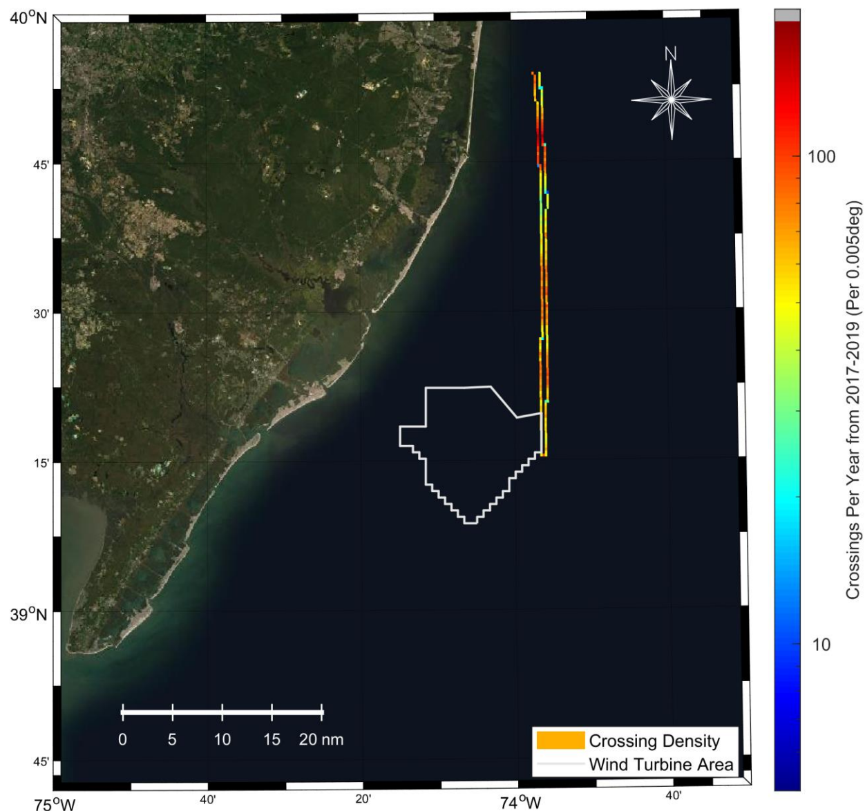
Figure 6.24: Track Density Map for Vessels Crossing the Monmouth ECC
