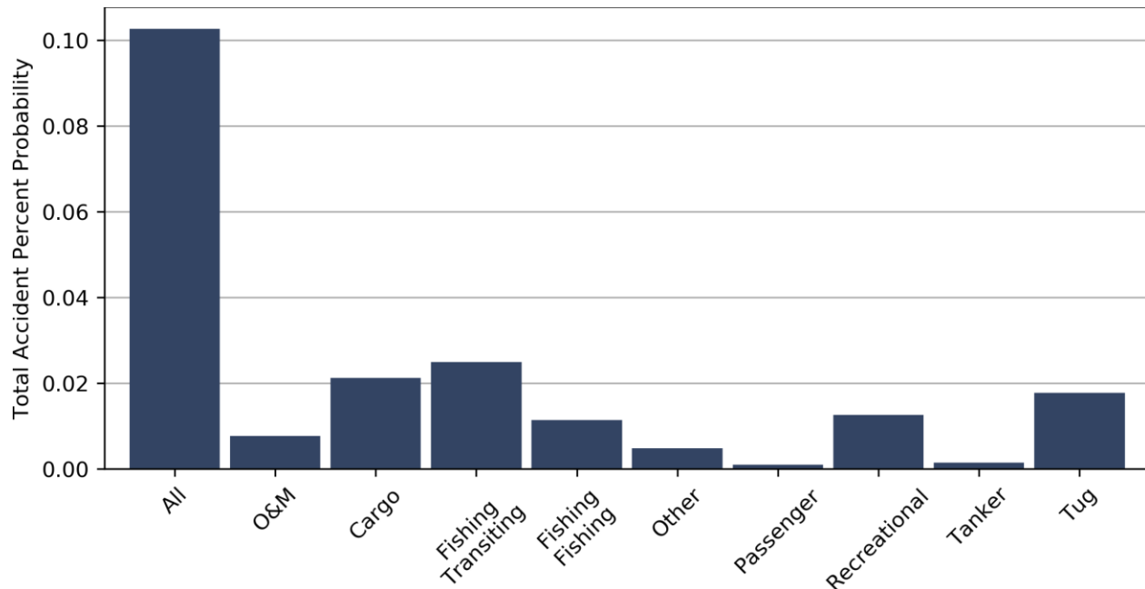
Figure 8.9: Estimated Operational Phase Inter-Class Accident Annual Frequencies
