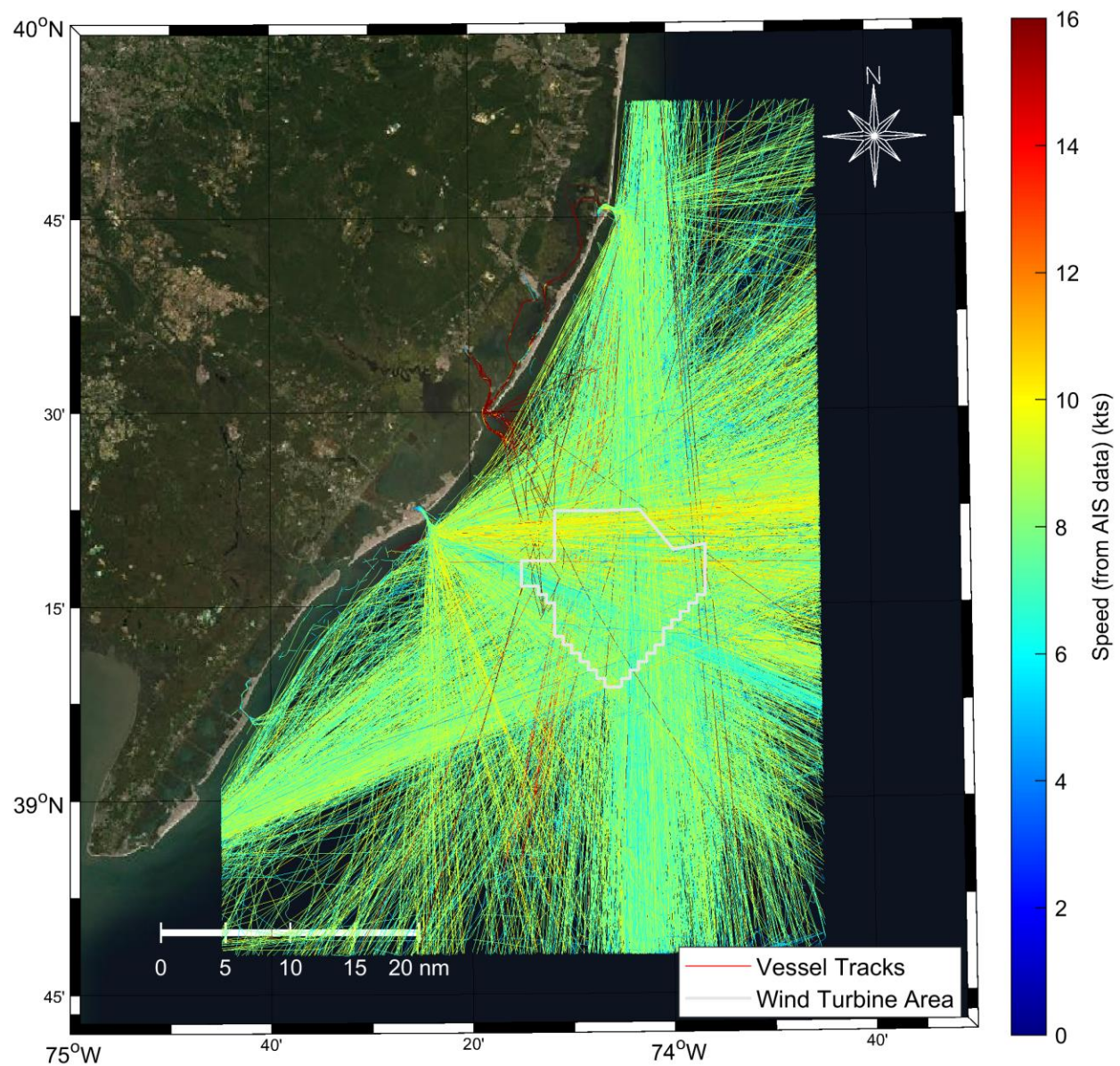
Figure C.18: Fishing Vessel Tracks Transiting Through the WTA (>4 Kts)
