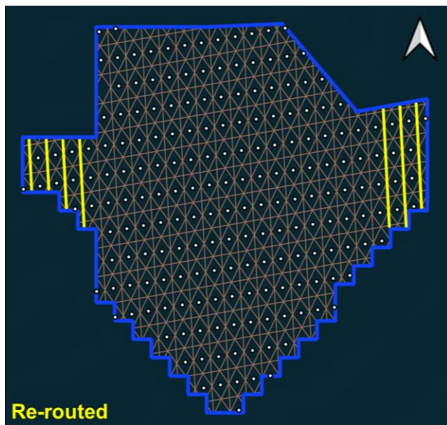
Figure 8.7: Re-routed N/S Corridors
