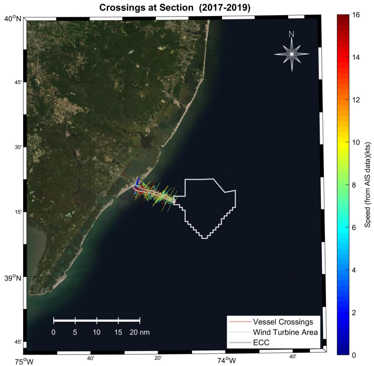
Figure 6.25: Vessel Tracks for Vessels Crossing the Atlantic ECC
