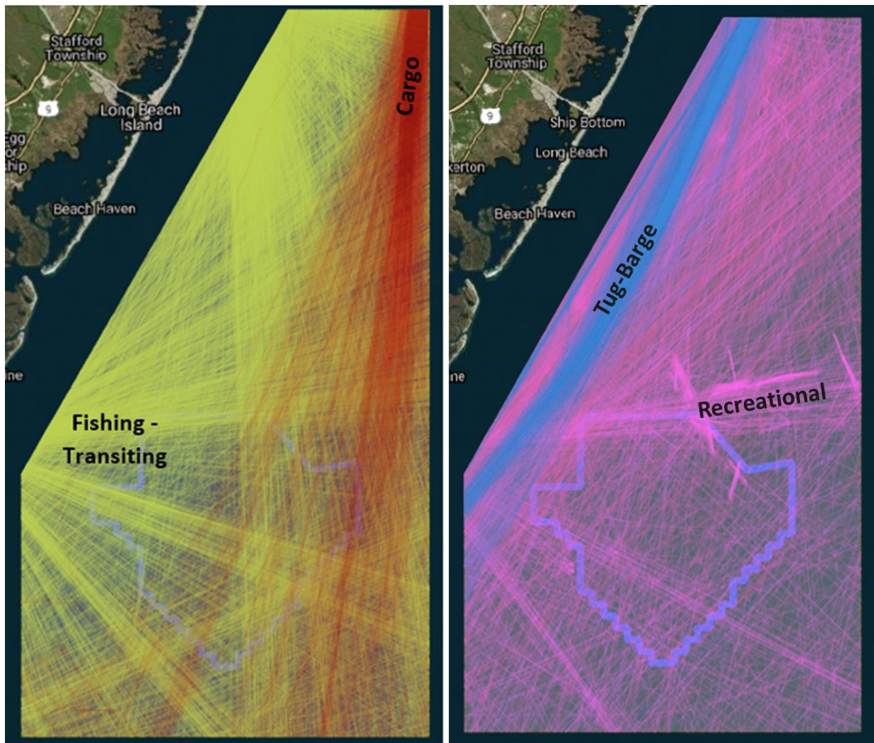
Figure 8.10: Tracks for Fishing (yellow), Cargo (red), Tug-Barge (blue), Recreational (magenta) Vessels
