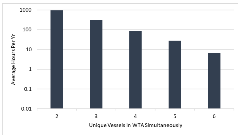
Figure 6.27: Histogram of Unique AIS Vessels in the WTA Per Year (Logarithmic Y-Axis)
