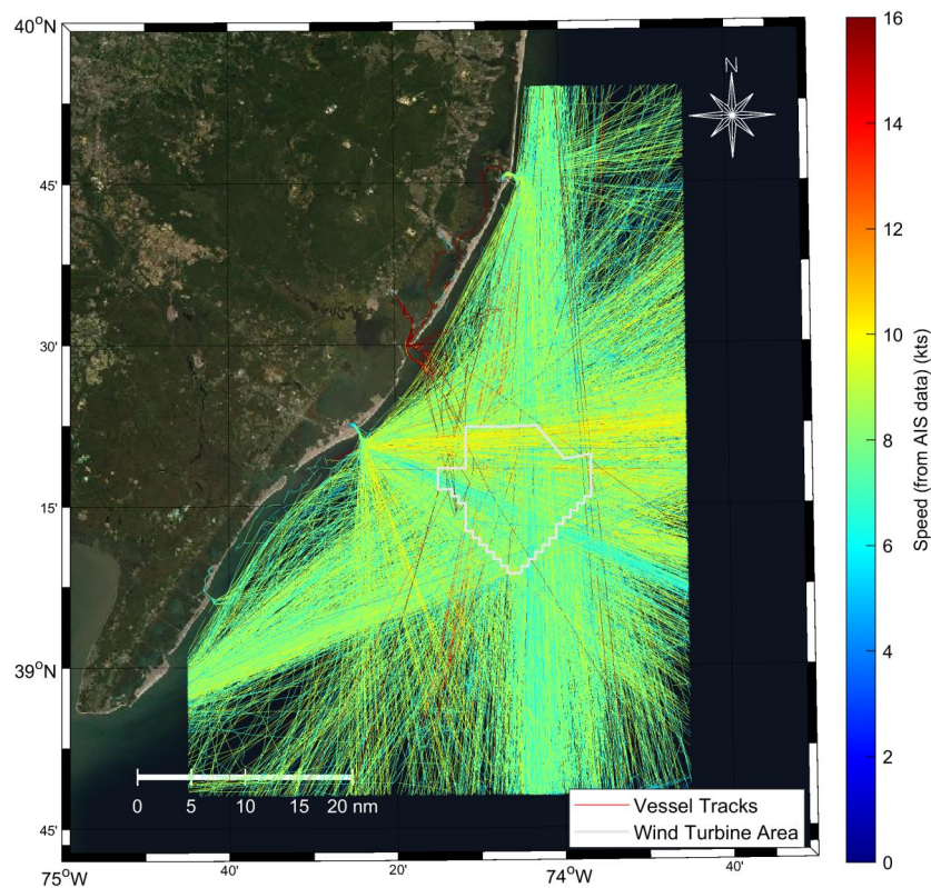
Figure 6.14: Fishing Vessel Tracks Transiting Through the WTA (>4 Kts)
