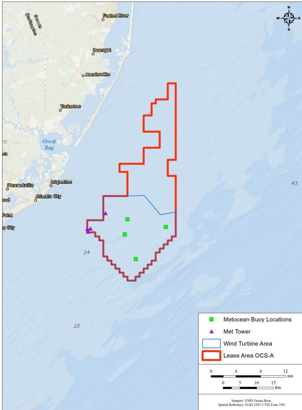
Figure 2.5: Potential Met Tower and Metocean Buoy Locations
