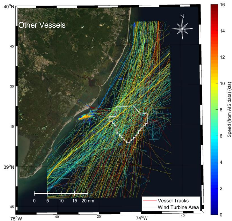
Figure 6.6: Tracks for “Other” Vessels Entering the WTA
