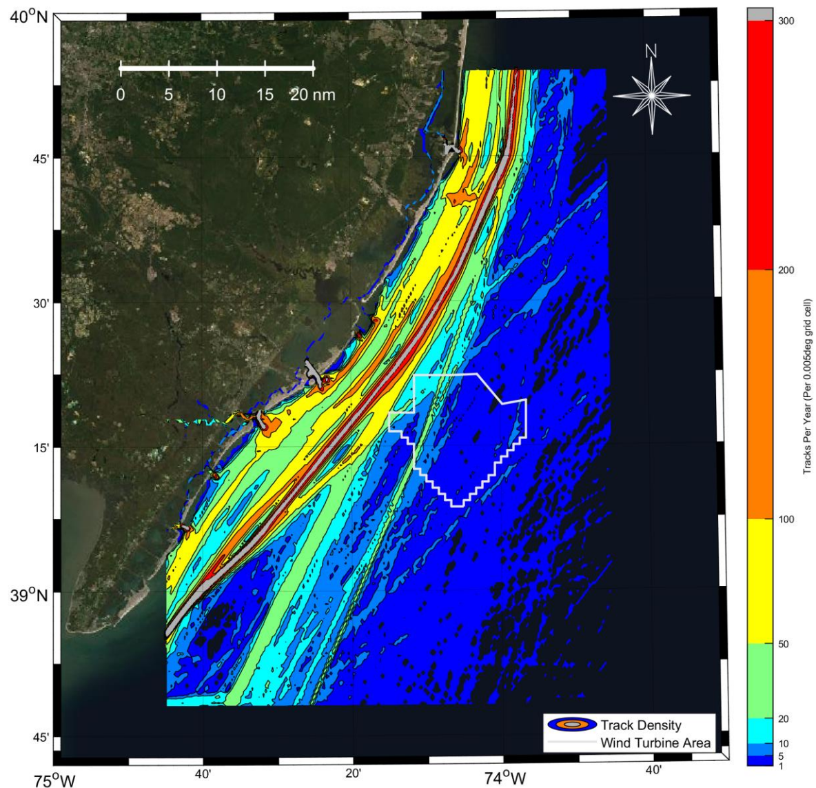
Figure 6.8: AIS Vessel Traffic Density for Tug Tows
