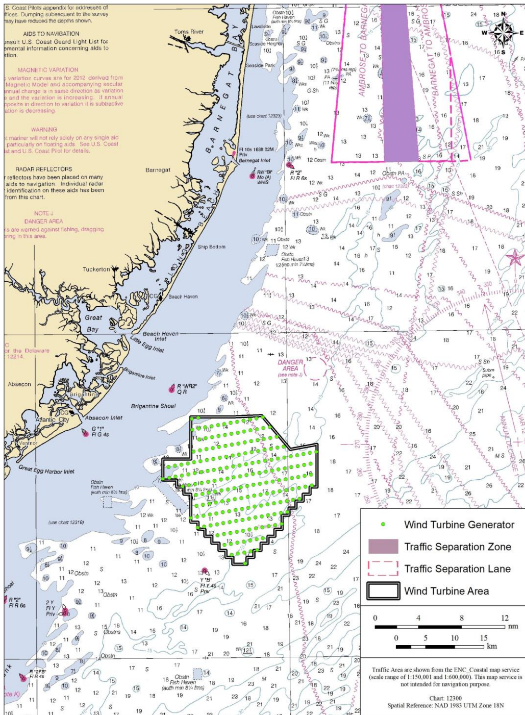
Figure 5.1: WTA Overlaid on Navigational Chart 12300
