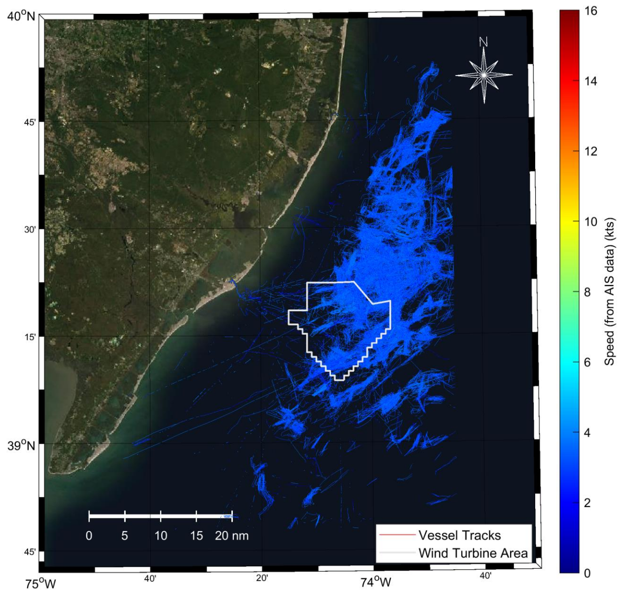
Figure C.17: Fishing Vessel Tracks Through the WTA Fishing (<4 Kts)
