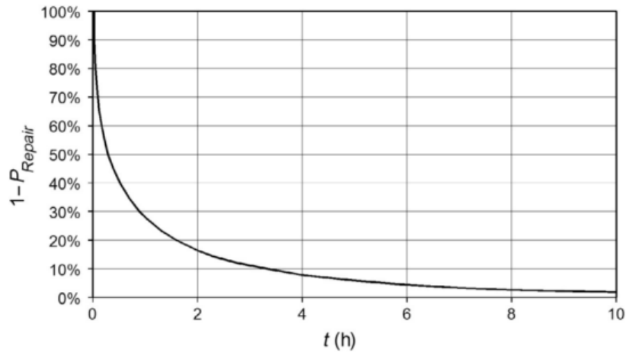
Figure E.8: Drift-repair function used in NORM (image adopted from Zhang et al., 2019)
