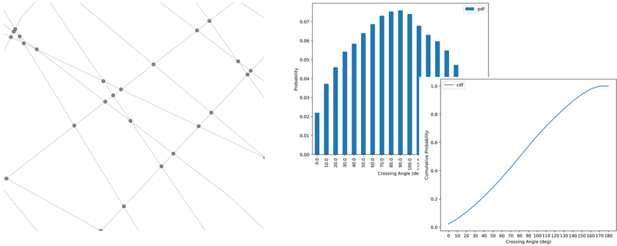
Figure E.4: AIS Tracks, and Track Intersection Angle Distribution
