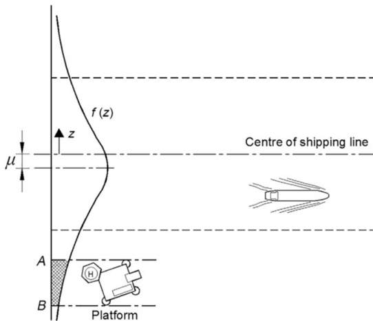
Figure E.7: Allision scenarios considered by NORM (Powered Allision image adopted from Zhang et al., 2019)
