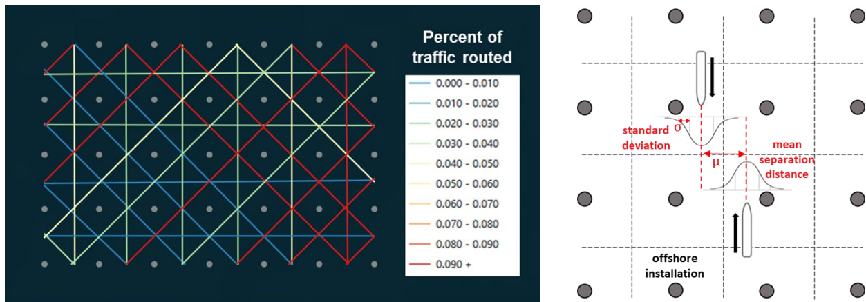
Figure E.5: Traffic routed through Turbine Field (left), Assumed Future Traffic (right)
