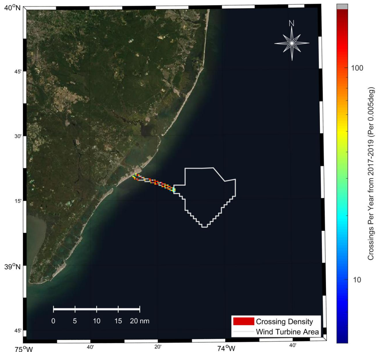
Figure 6.26: Track Density for Vessels Crossing the Atlantic ECC
