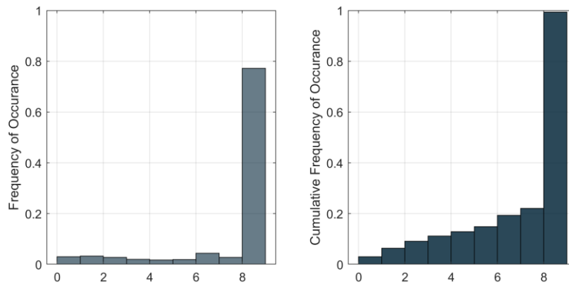
Figure 4.5: Observed 2000-2019 visibility at Atlantic City Airport (ACY)
