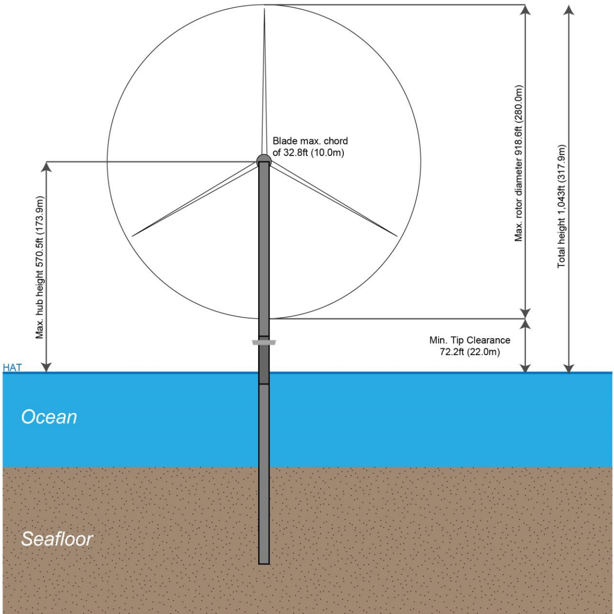
Figure 8.11: WTG Maximum Dimensions and Minimum Vertical Clearance of the Blade Tip Above the Water Surface
