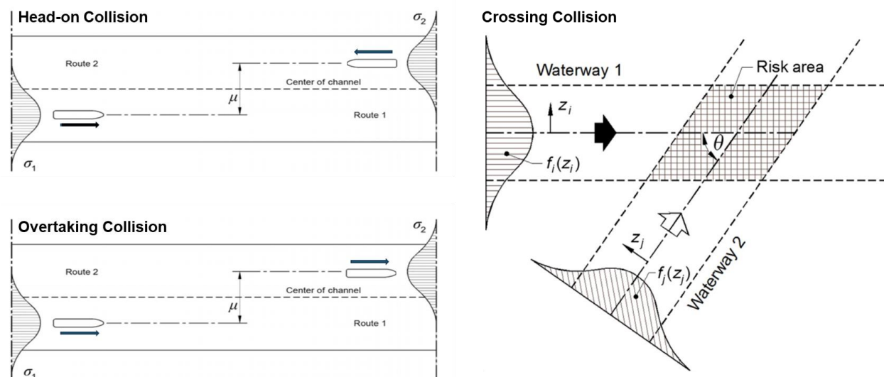
Figure E.6: Collision Scenarios considered by NORM (images adopted from Zhang et al., 2019)
