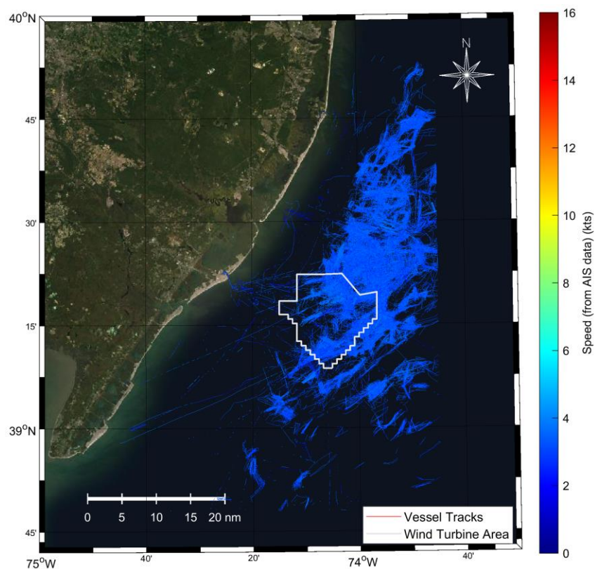
Figure 6.13: Fishing Vessel Tracks Through the WTA Fishing (<4 Kts)
