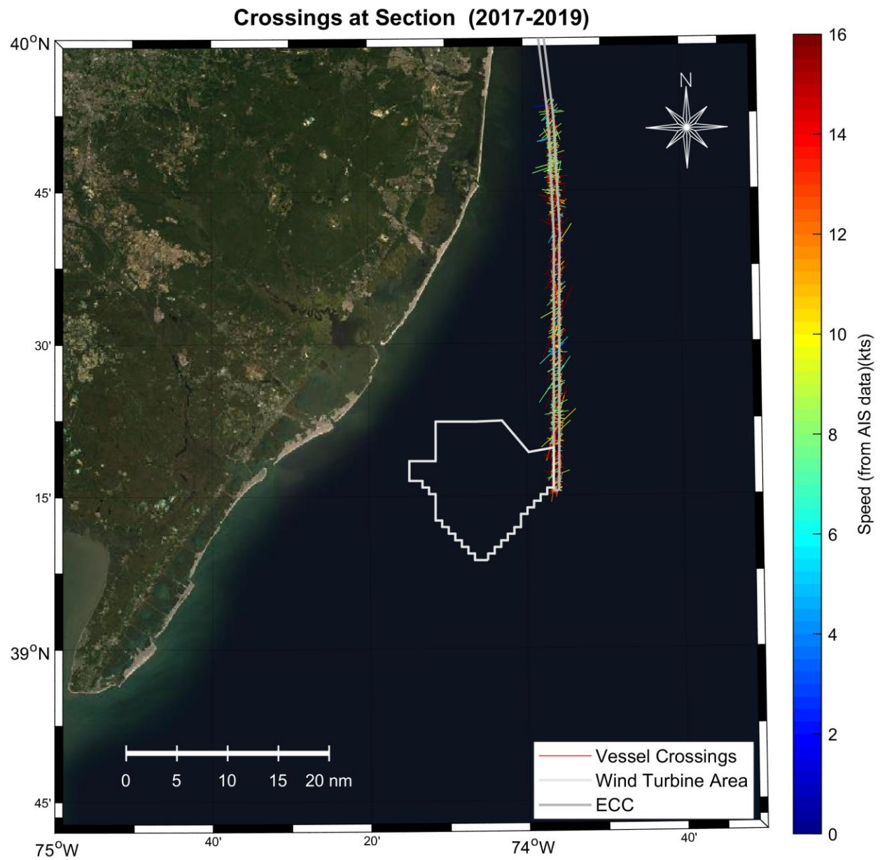
Figure 6.23: Vessel Tracks for Vessels Crossing the Monmouth ECC
