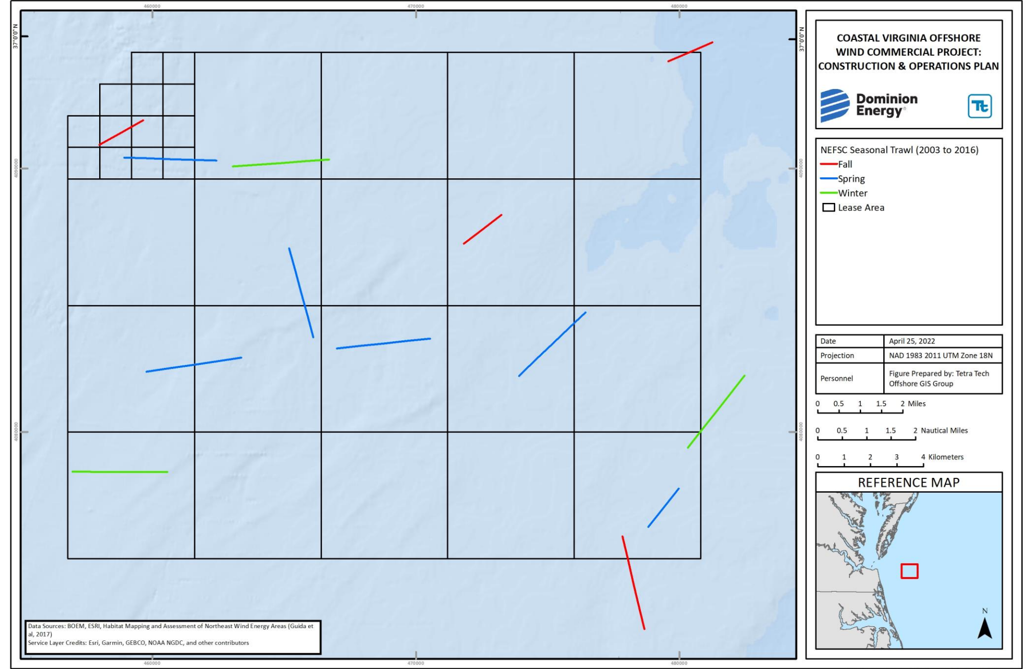
Figure 4.2-18. Locations of NEFSC Seasonal Trawls from 2003 to 2016 (from Guida et al. 2017)
