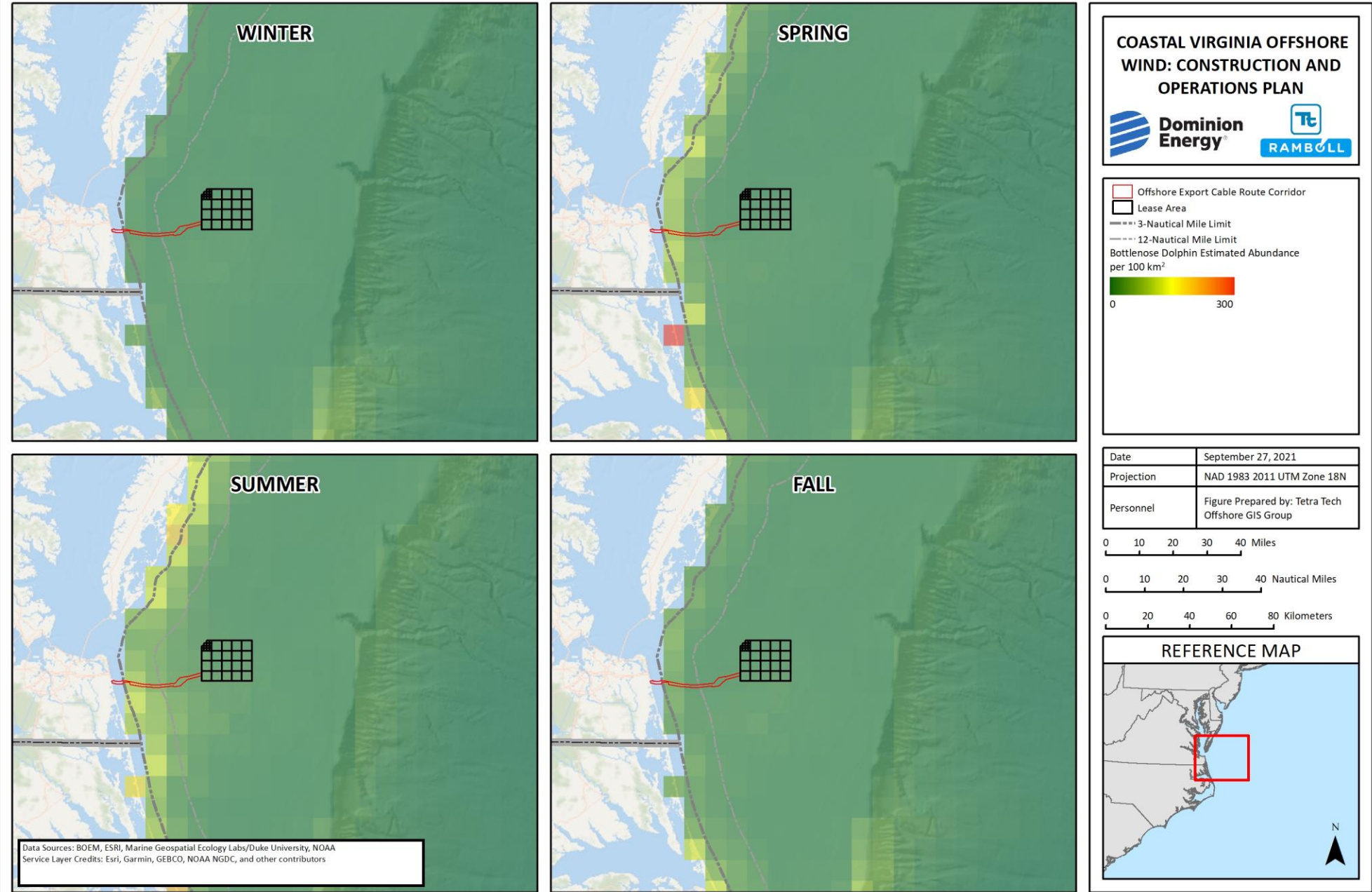
Figure 4.2-31. Seasonal Distribution of the Bottlenose Dolphin in the Marine Mammal Study Area
