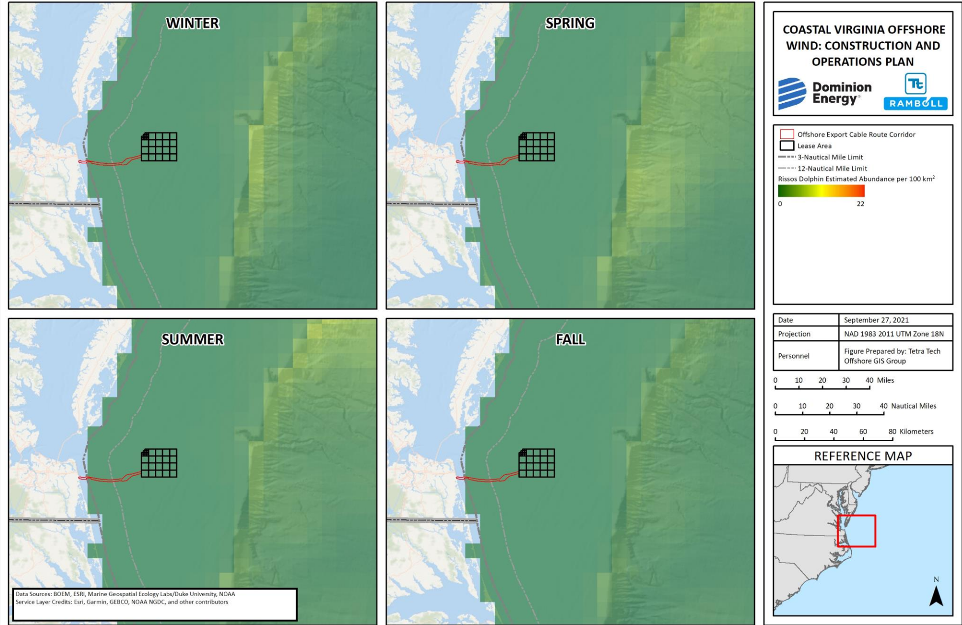
Figure 4.2-34. Seasonal Distribution of the Risso's Dolphin in the Marine Mammal Study Area
