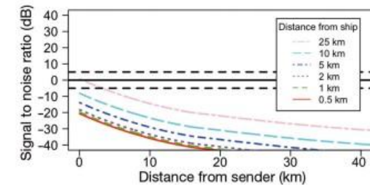
Fig. 2. Detection ranges of the North Atlantic right whale Eubalaena glacialis upcall by a receiver at 0.5, 1, 2, 5, 10, and 25 km from point-source noise produced by a container ship. Horizontal black lines correspond to receiver critical ratios of 0 dB (solid) and \pm 5 dB (dashed). For a critical ratio of 0 dB, detection of an upcall would only occur at 25 km from a container ship. For a critical ratio of 5 dB, signal detection would fail in all scenarios modeled, at all distances from a signaling whale
