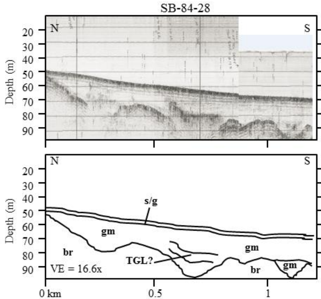
Figure C2. Seismic profile SB-84-28. Representative profile for zone F. Estimated mean thickness for uppermost Holocene sand was 2 m. Samples collected in this unit contained 62% to 92% fine sand with considerable proportions of mud.
