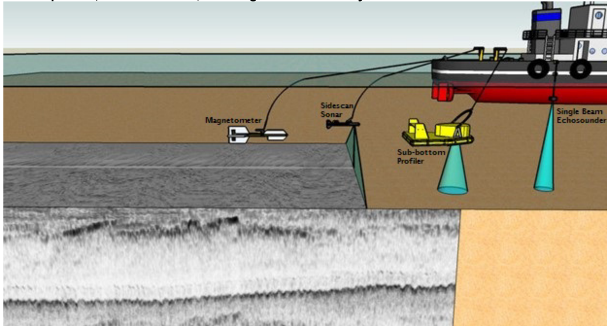
Figure 31: Schematic diagram showing the typical deployment of sensors: joint bathymetric, sub-bottom profiler, sidescan sonar, and magnetometer survey.
