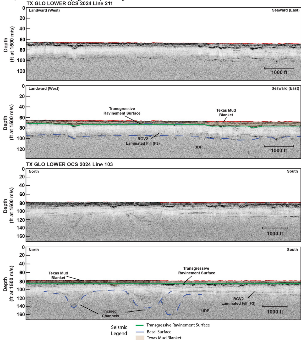
Figure 48: Seismic examples of the Rio Grande Incised Valley fill 2 (Feature 3).
