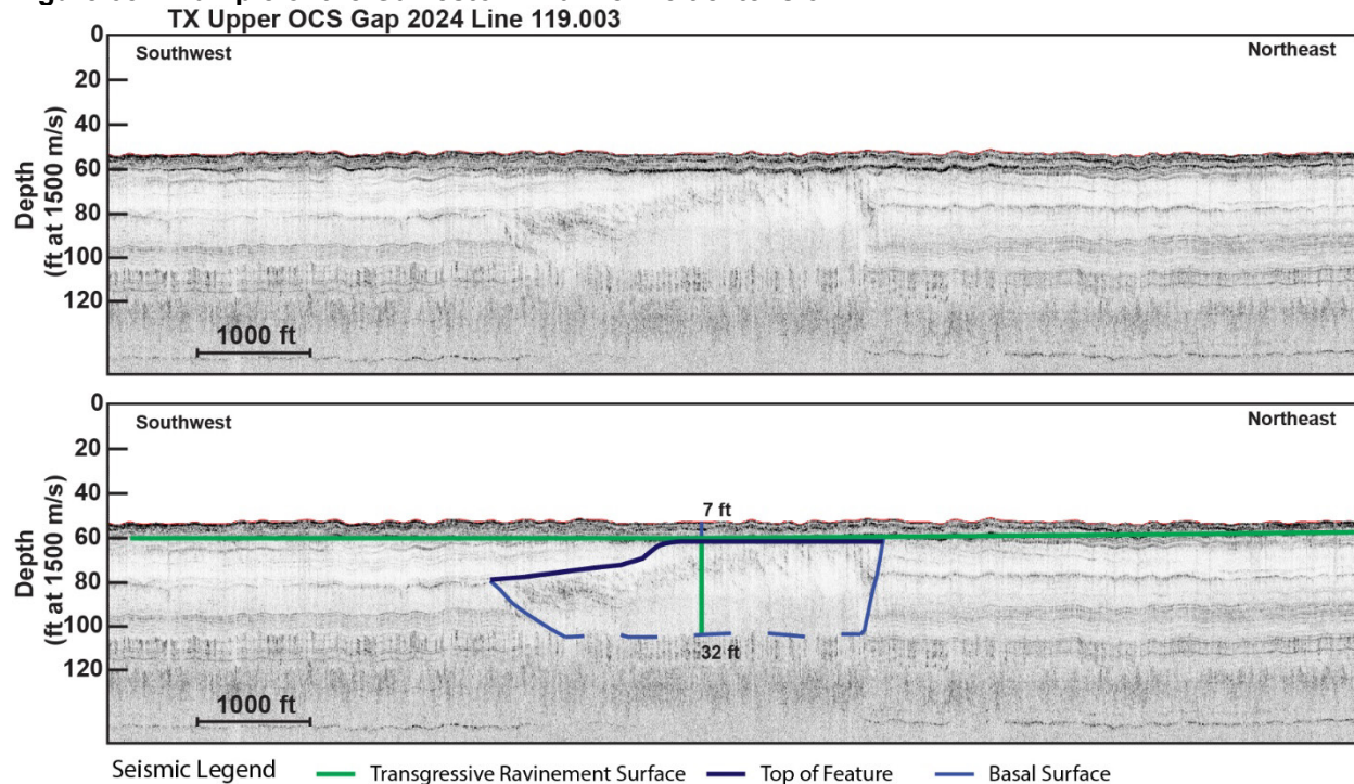
Figure 68: Example of the Galveston Channel Belt extension.
