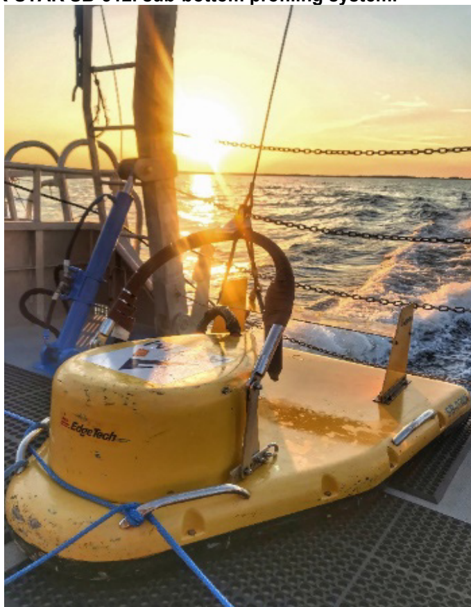
Figure 34: EdgeTech X-STAR SB-512i sub-bottom profiling system.
