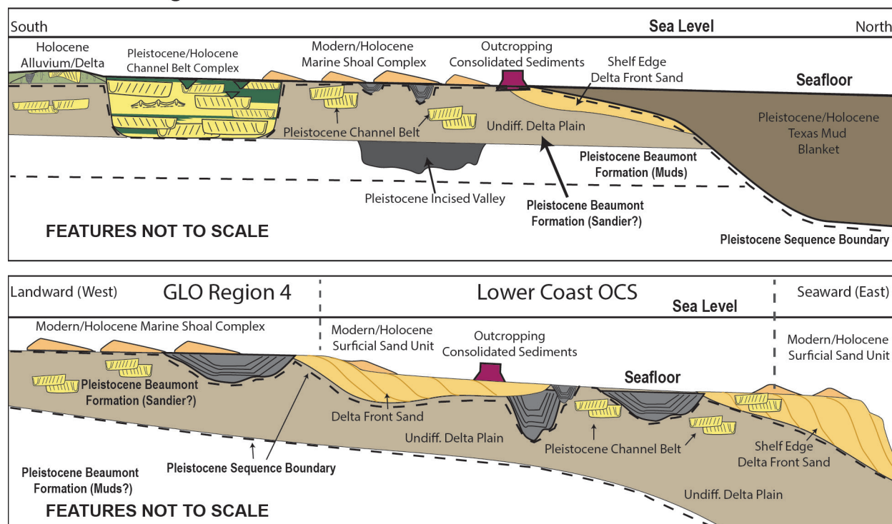
Figure 56: Generalized cross-section of major features observed in the GLO Region 4 and Lower OCS Investigation Area.
