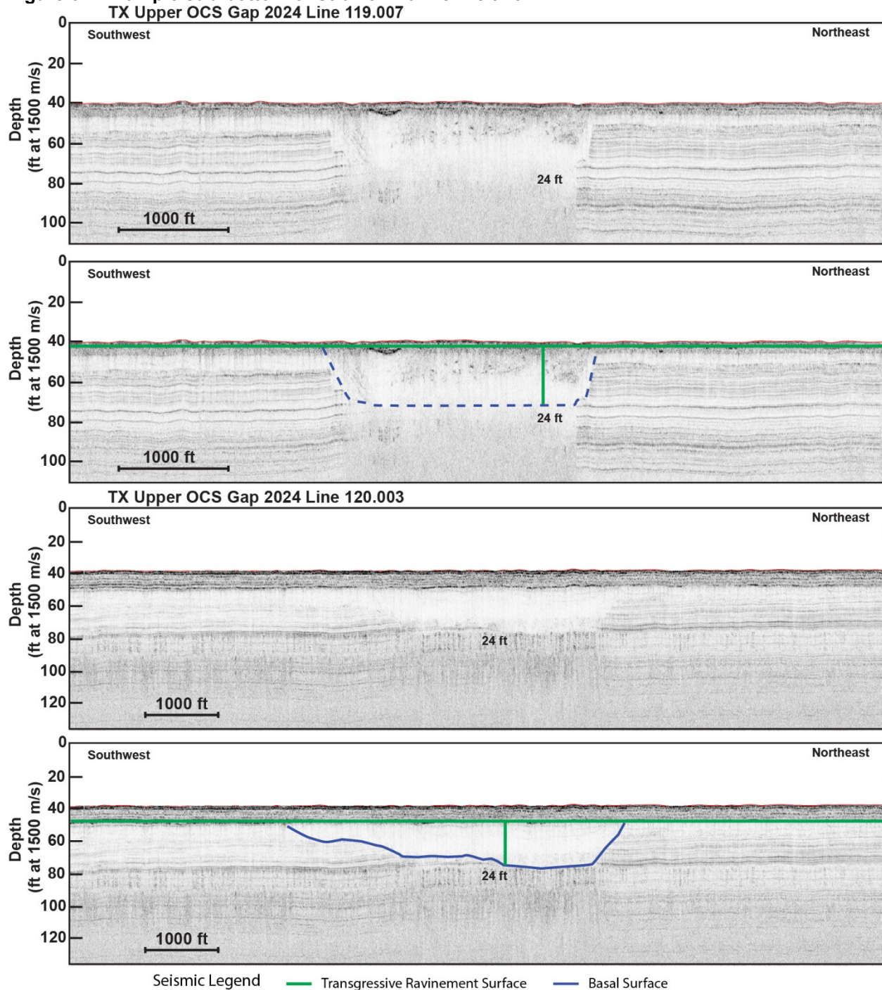
Figure 64: Example sub-bottom of Sabine Channel Belt 10.
