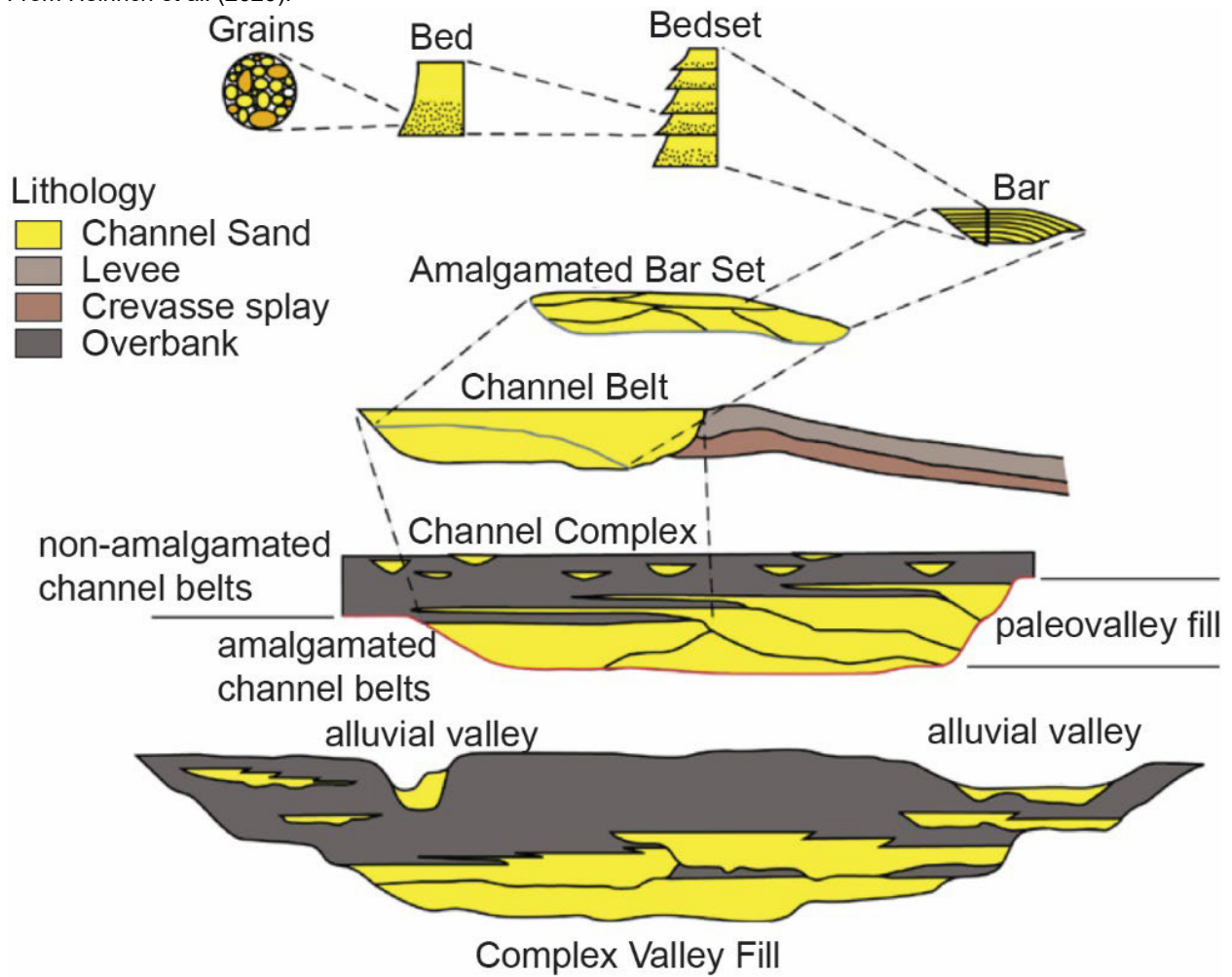
Figure 22: Conceptual hierarchy of fluvial deposits.
