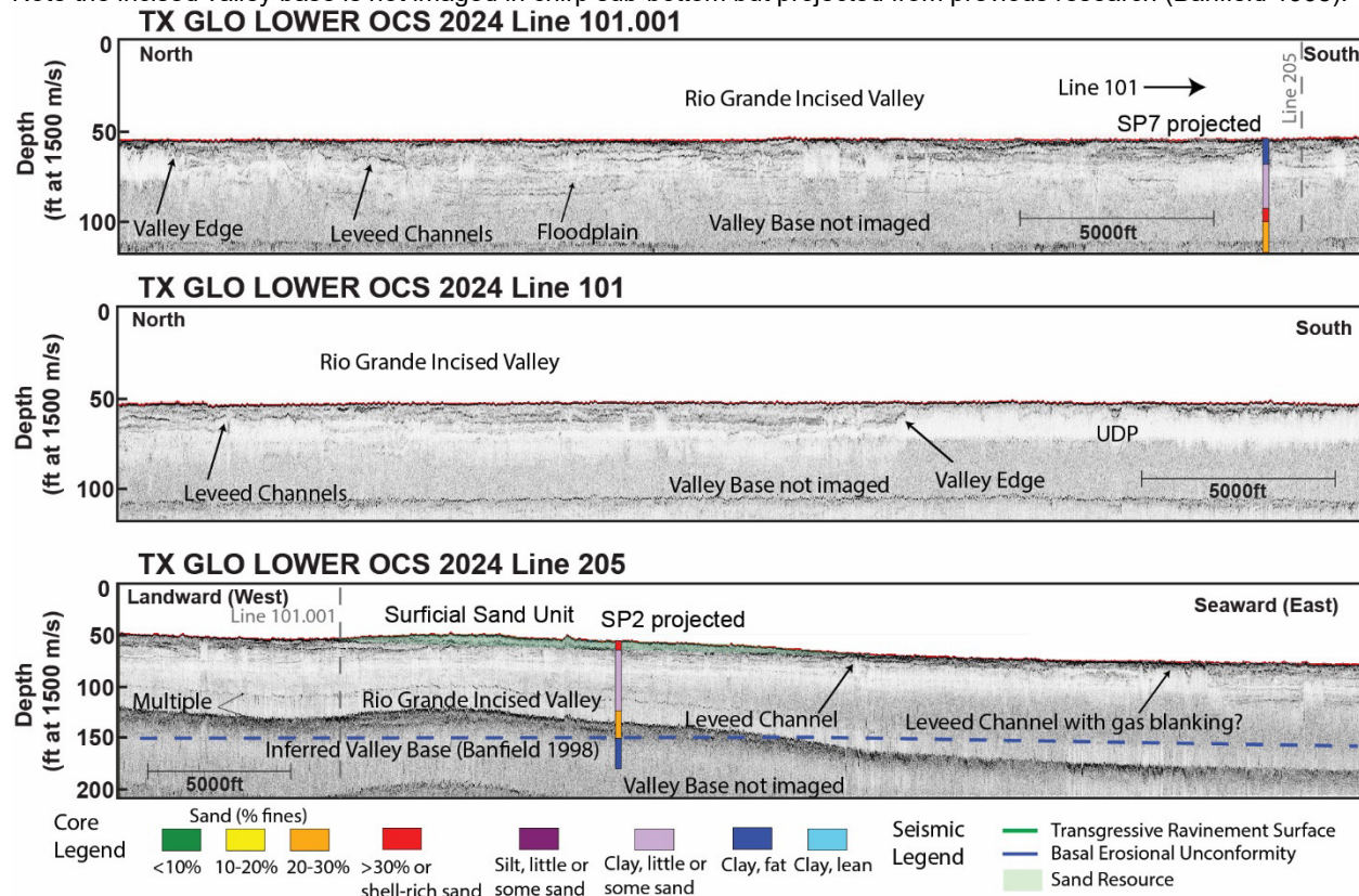
Figure 51: Examples of the Rio Grande Incised Valley, fill, and overlying surficial sand unit.
