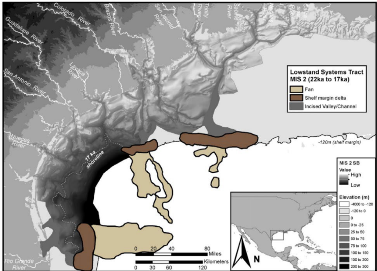
Figure 13: Lowstand valleys and fans of the Southern Texas systems. From Anderson et al. (2016).
