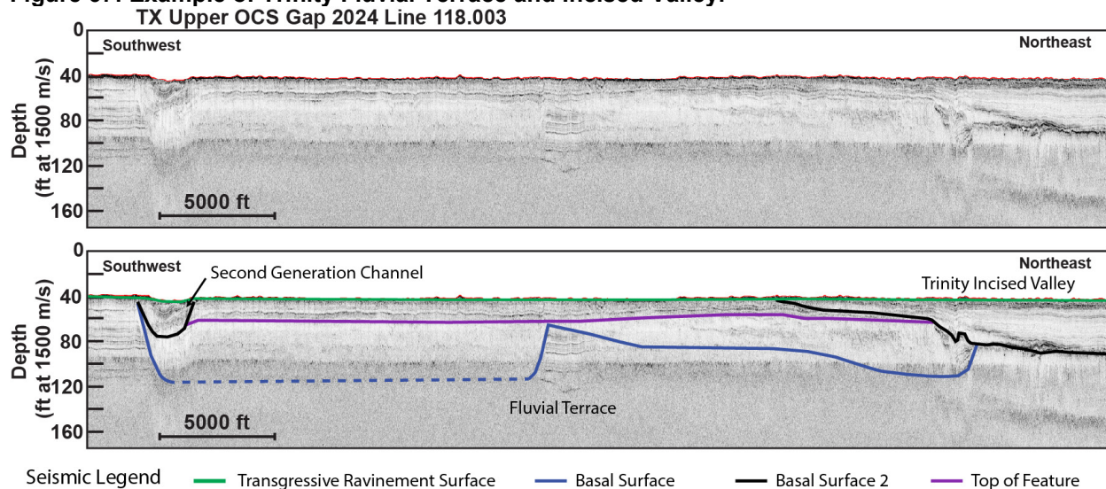
Figure 67: Example of Trinity Fluvial Terrace and Incised Valley.
